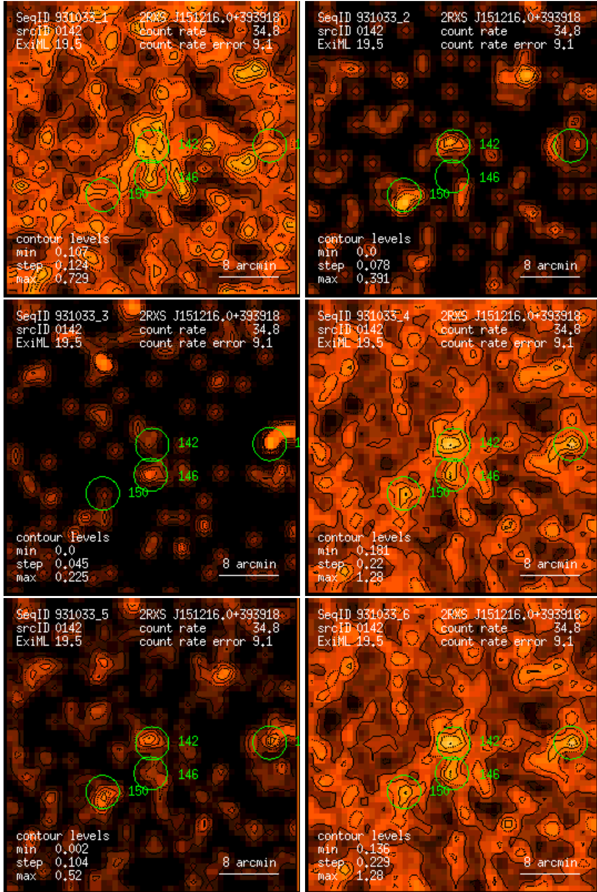
Figure 142: RASS 931033: detection 0142: band rate images, Gaussian filter: (1) PSPC channels 11 – 41, (2) 52 – 90, (3) 91 – 201, (4) 11 – 235, (5) 52 – 201, (6) 11 – 201. Broad band rates in counts/ks. Band rate contour levels in counts/ks/arcmin 2 .
