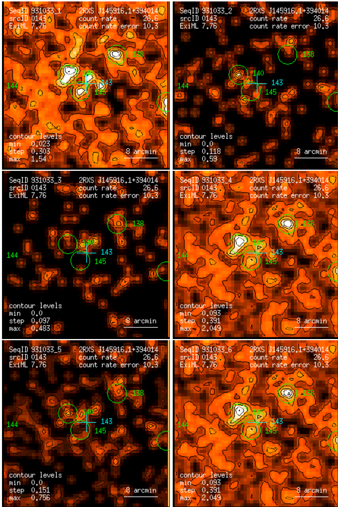
Figure 143: RASS 931033: detection 0143: band rate images, Gaussian filter: (1) PSPC channels 11 – 41, (2) 52 – 90, (3) 91 – 201, (4) 11 – 235, (5) 52 – 201, (6) 11 – 201. Broad band rates in counts/ks. Band rate contour levels in counts/ks/arcmin 2 .
