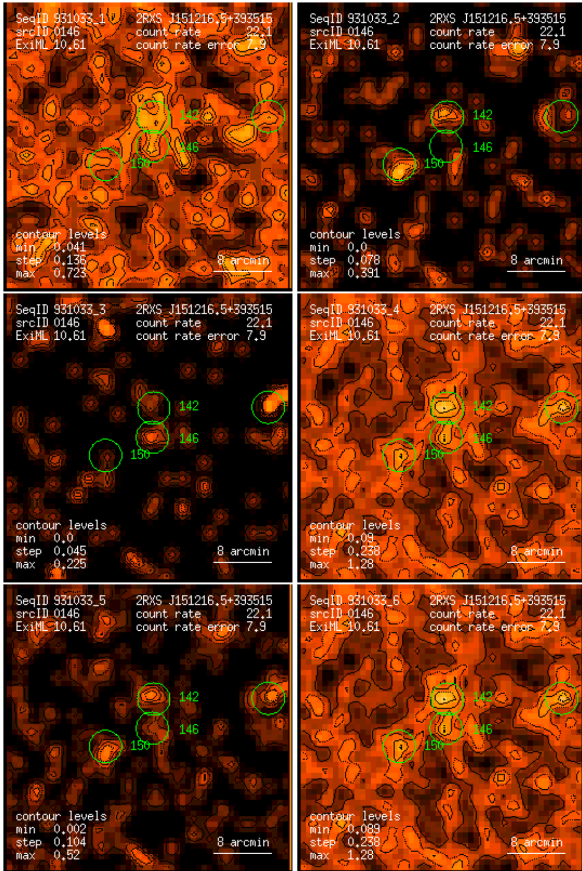
Figure 146: RASS 931033: detection 0146: band rate images, Gaussian filter: (1) PSPC channels 11 – 41, (2) 52 – 90, (3) 91 – 201, (4) 11 – 235, (5) 52 – 201, (6) 11 – 201. Broad band rates in counts/ks. Band rate contour levels in counts/ks/arcmin 2 .
