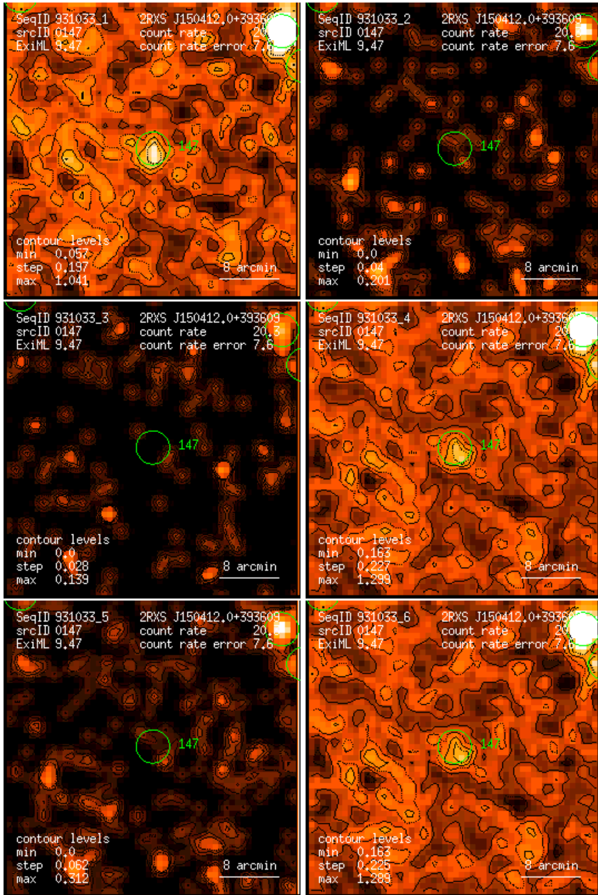
Figure 147: RASS 931033: detection 0147: band rate images, Gaussian filter: (1) PSPC channels 11 – 41, (2) 52 – 90, (3) 91 – 201, (4) 11 – 235, (5) 52 – 201, (6) 11 – 201. Broad band rates in counts/ks. Band rate contour levels in counts/ks/arcmin 2 .
