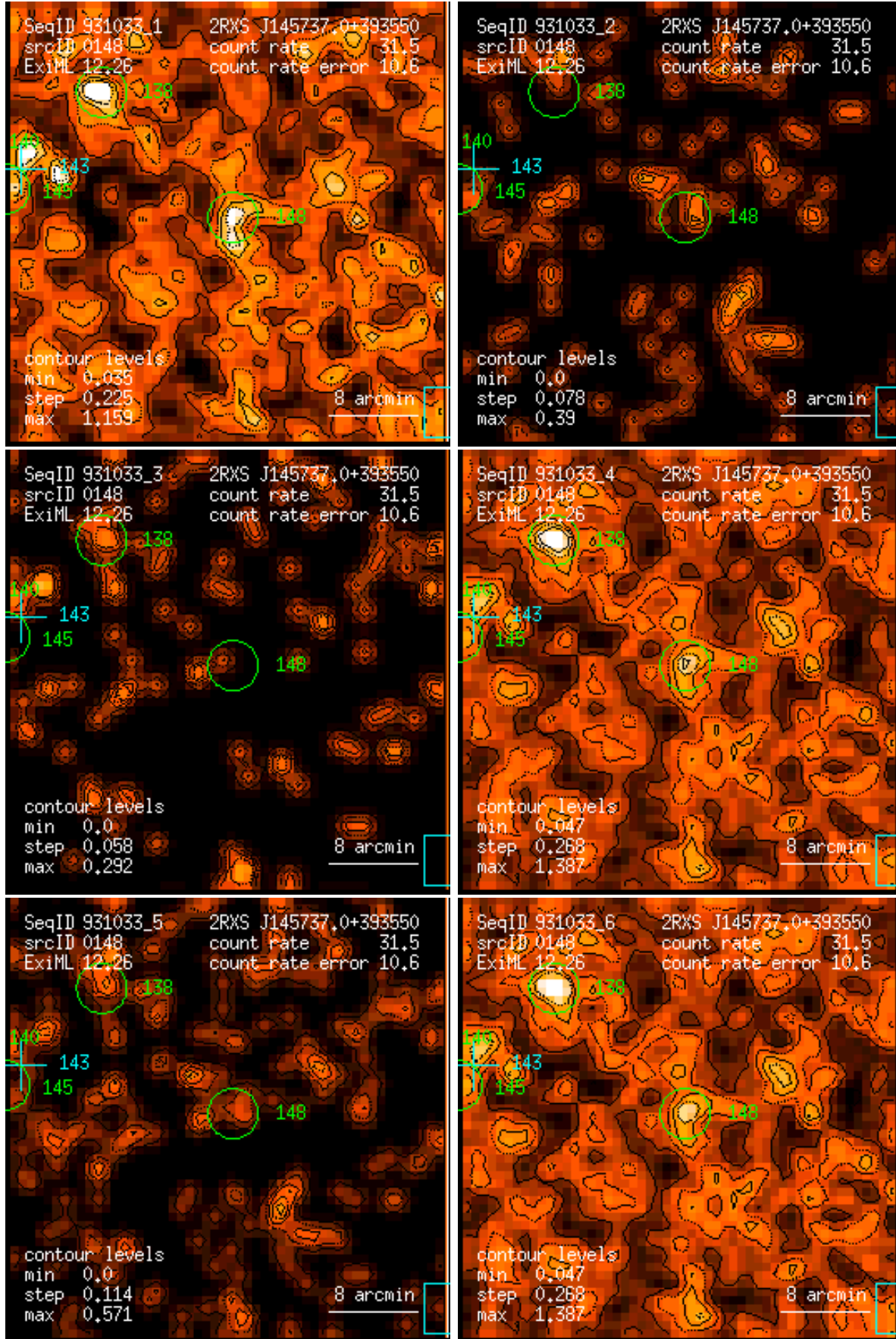
Figure 148: RASS 931033: detection 0148: band rate images, Gaussian filter: (1) PSPC channels 11 – 41, (2) 52 – 90, (3) 91 – 201, (4) 11 – 235, (5) 52 – 201, (6) 11 – 201. Broad band rates in counts/ks. Band rate contour levels in counts/ks/arcmin 2 .
