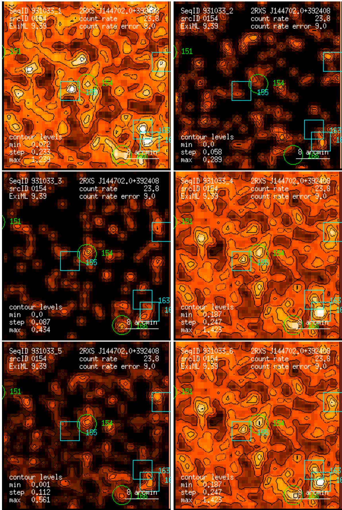
Figure 154: RASS 931033: detection 0154: band rate images, Gaussian filter: (1) PSPC channels 11 – 41, (2) 52 – 90, (3) 91 – 201, (4) 11 – 235, (5) 52 – 201, (6) 11 – 201. Broad band rates in counts/ks. Band rate contour levels in counts/ks/arcmin 2 .
