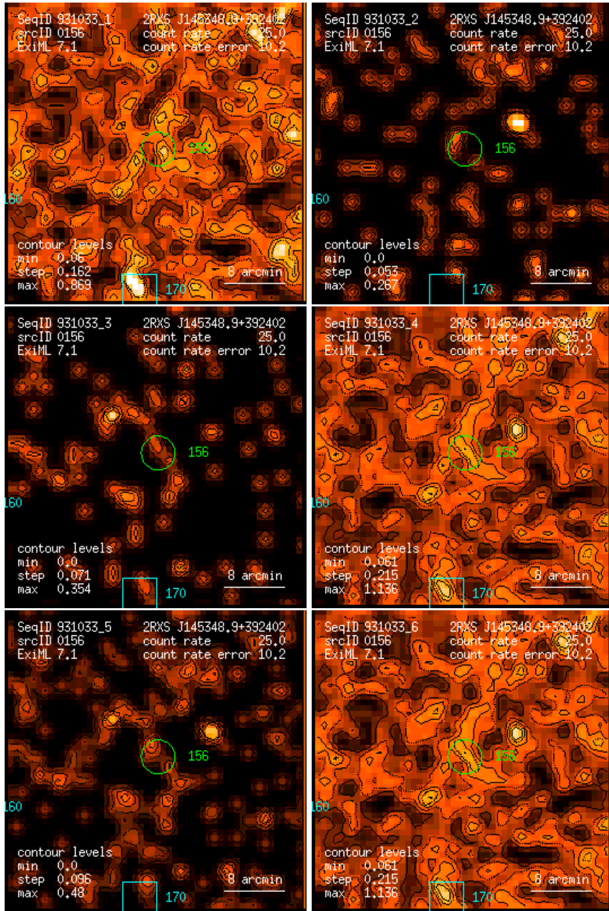
Figure 156: RASS 931033: detection 0156: band rate images, Gaussian filter: (1) PSPC channels 11 – 41, (2) 52 – 90, (3) 91 – 201, (4) 11 – 235, (5) 52 – 201, (6) 11 – 201. Broad band rates in counts/ks. Band rate contour levels in counts/ks/arcmin 2 .
