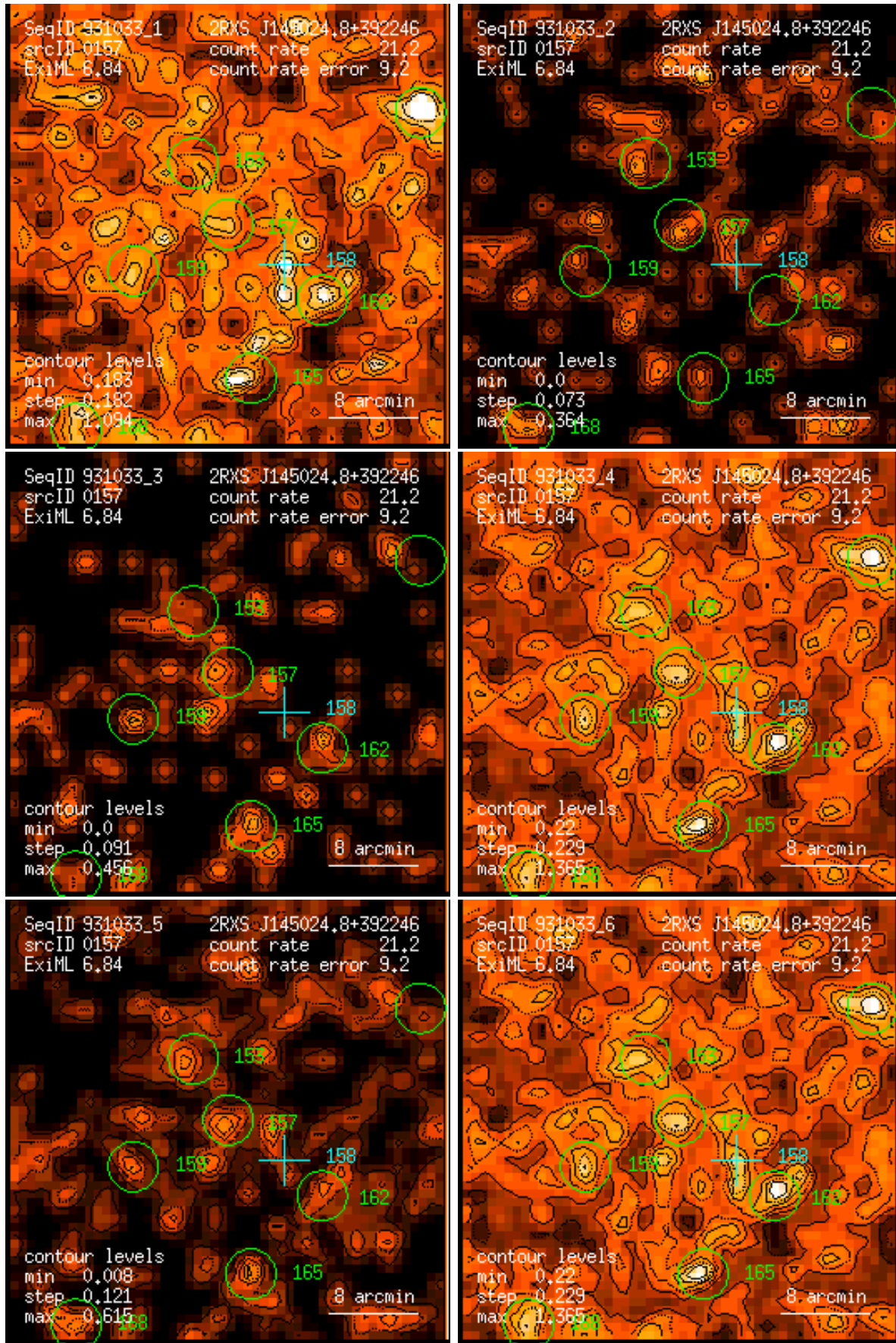
Figure 157: RASS 931033: detection 0157: band rate images, Gaussian filter: (1) PSPC channels 11 – 41, (2) 52 – 90, (3) 91 – 201, (4) 11 – 235, (5) 52 – 201, (6) 11 – 201. Broad band rates in counts/ks. Band rate contour levels in counts/ks/arcmin 2 .
