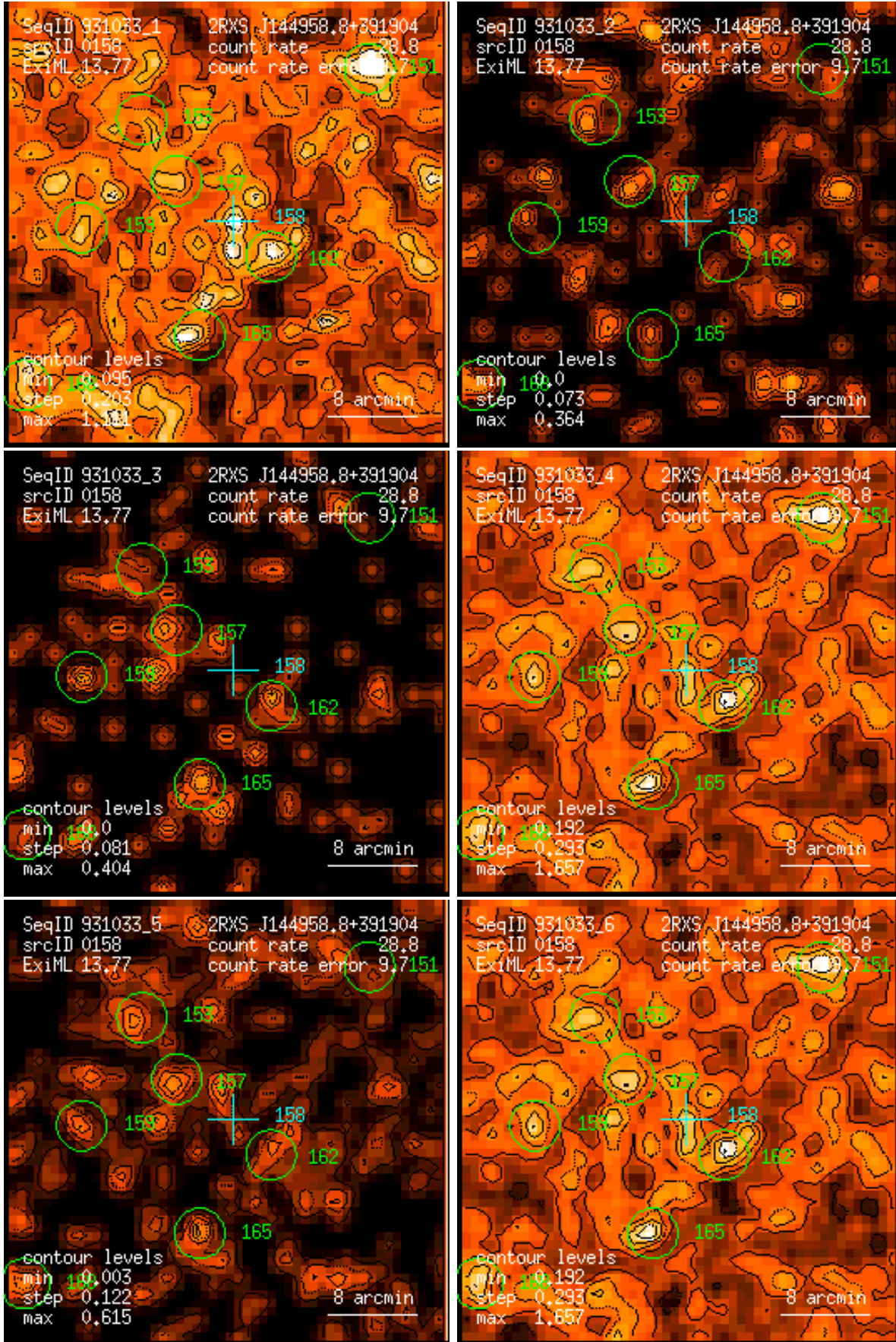
Figure 158: RASS 931033: detection 0158: band rate images, Gaussian filter: (1) PSPC channels 11 – 41, (2) 52 – 90, (3) 91 – 201, (4) 11 – 235, (5) 52 – 201, (6) 11 – 201. Broad band rates in counts/ks. Band rate contour levels in counts/ks/arcmin 2 .
