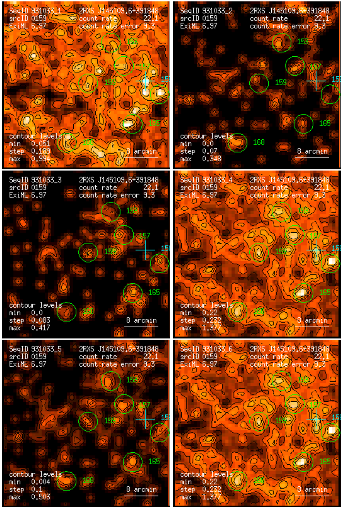
Figure 159: RASS 931033: detection 0159: band rate images, Gaussian filter: (1) PSPC channels 11 – 41, (2) 52 – 90, (3) 91 – 201, (4) 11 – 235, (5) 52 – 201, (6) 11 – 201. Broad band rates in counts/ks. Band rate contour levels in counts/ks/arcmin 2 .
