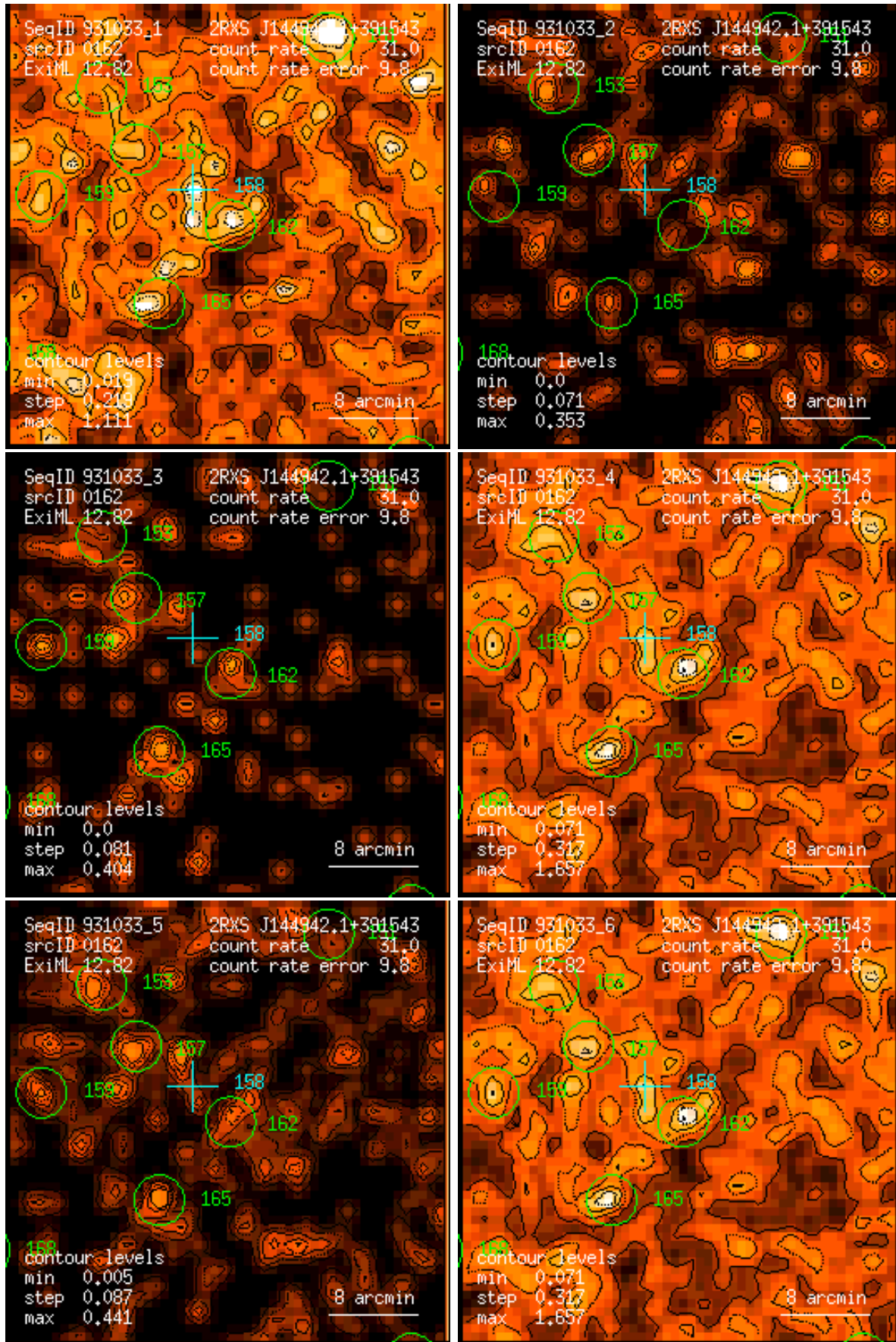
Figure 162: RASS 931033: detection 0162: band rate images, Gaussian filter: (1) PSPC channels 11 – 41, (2) 52 – 90, (3) 91 – 201, (4) 11 – 235, (5) 52 – 201, (6) 11 – 201. Broad band rates in counts/ks. Band rate contour levels in counts/ks/arcmin 2 .
