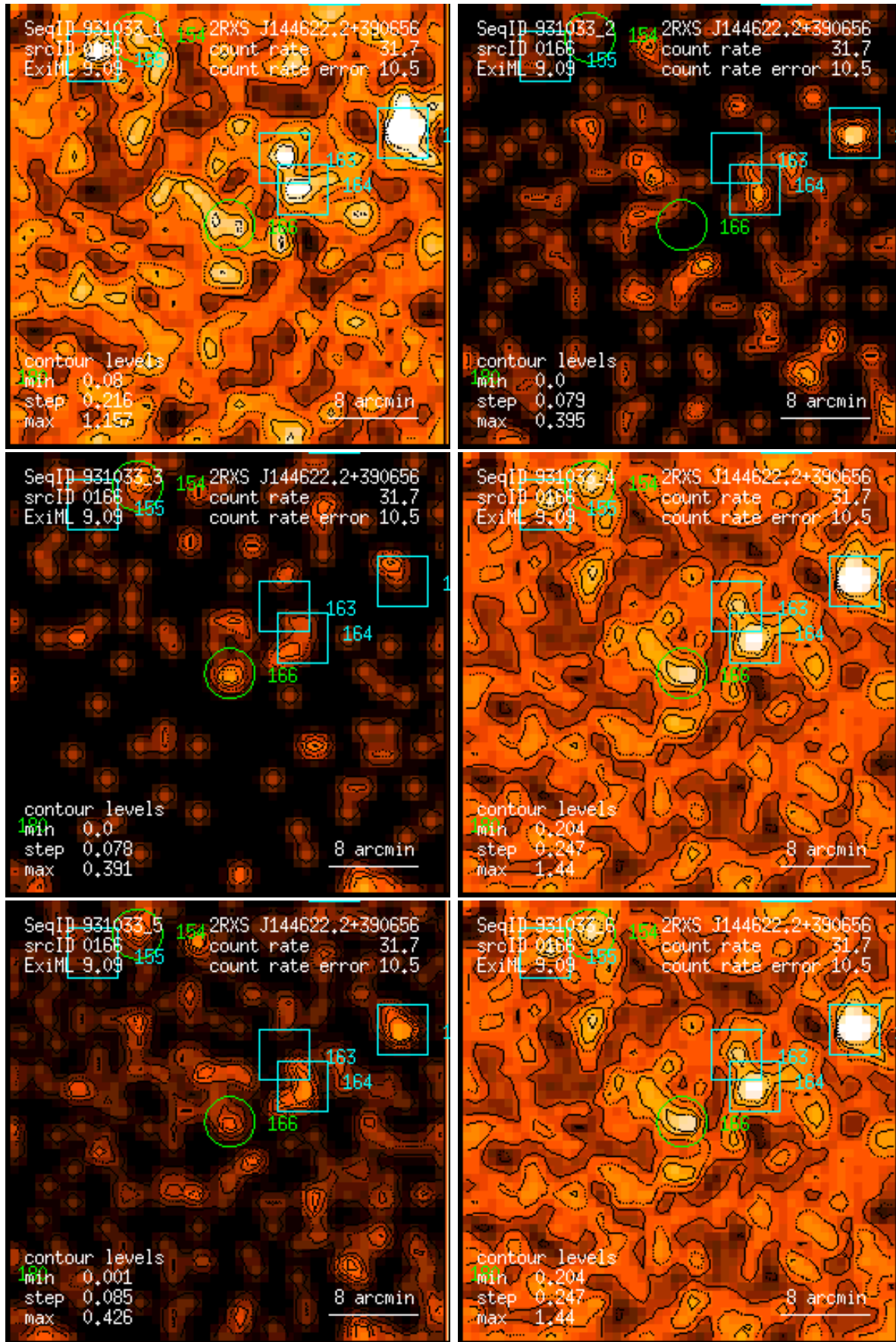
Figure 166: RASS 931033: detection 0166: band rate images, Gaussian filter: (1) PSPC channels 11 – 41, (2) 52 – 90, (3) 91 – 201, (4) 11 – 235, (5) 52 – 201, (6) 11 – 201. Broad band rates in counts/ks. Band rate contour levels in counts/ks/arcmin 2 .
