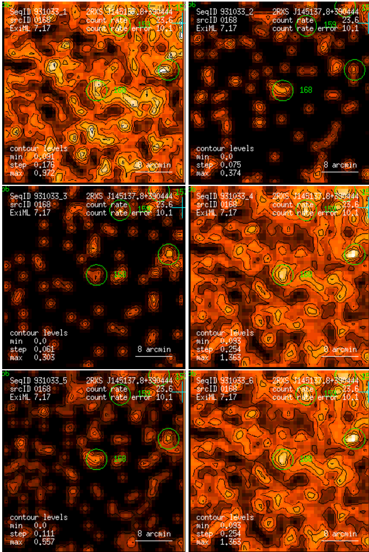
Figure 168: RASS 931033: detection 0168: band rate images, Gaussian filter: (1) PSPC channels 11 – 41, (2) 52 – 90, (3) 91 – 201, (4) 11 – 235, (5) 52 – 201, (6) 11 – 201. Broad band rates in counts/ks. Band rate contour levels in counts/ks/arcmin 2 .
