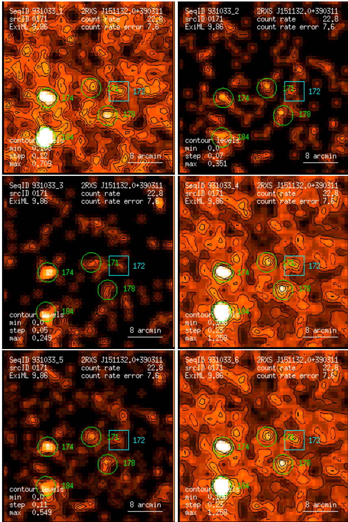
Figure 171: RASS 931033: detection 0171: band rate images, Gaussian filter: (1) PSPC channels 11 – 41, (2) 52 – 90, (3) 91 – 201, (4) 11 – 235, (5) 52 – 201, (6) 11 – 201. Broad band rates in counts/ks. Band rate contour levels in counts/ks/arcmin 2 .
