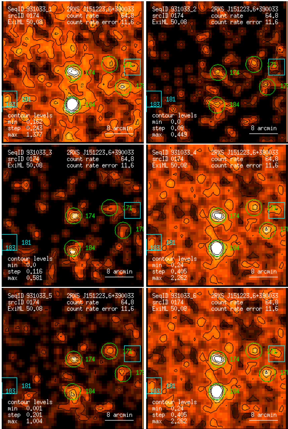
Figure 174: RASS 931033: detection 0174: band rate images, Gaussian filter: (1) PSPC channels 11 – 41, (2) 52 – 90, (3) 91 – 201, (4) 11 – 235, (5) 52 – 201, (6) 11 – 201. Broad band rates in counts/ks. Band rate contour levels in counts/ks/arcmin 2 .
