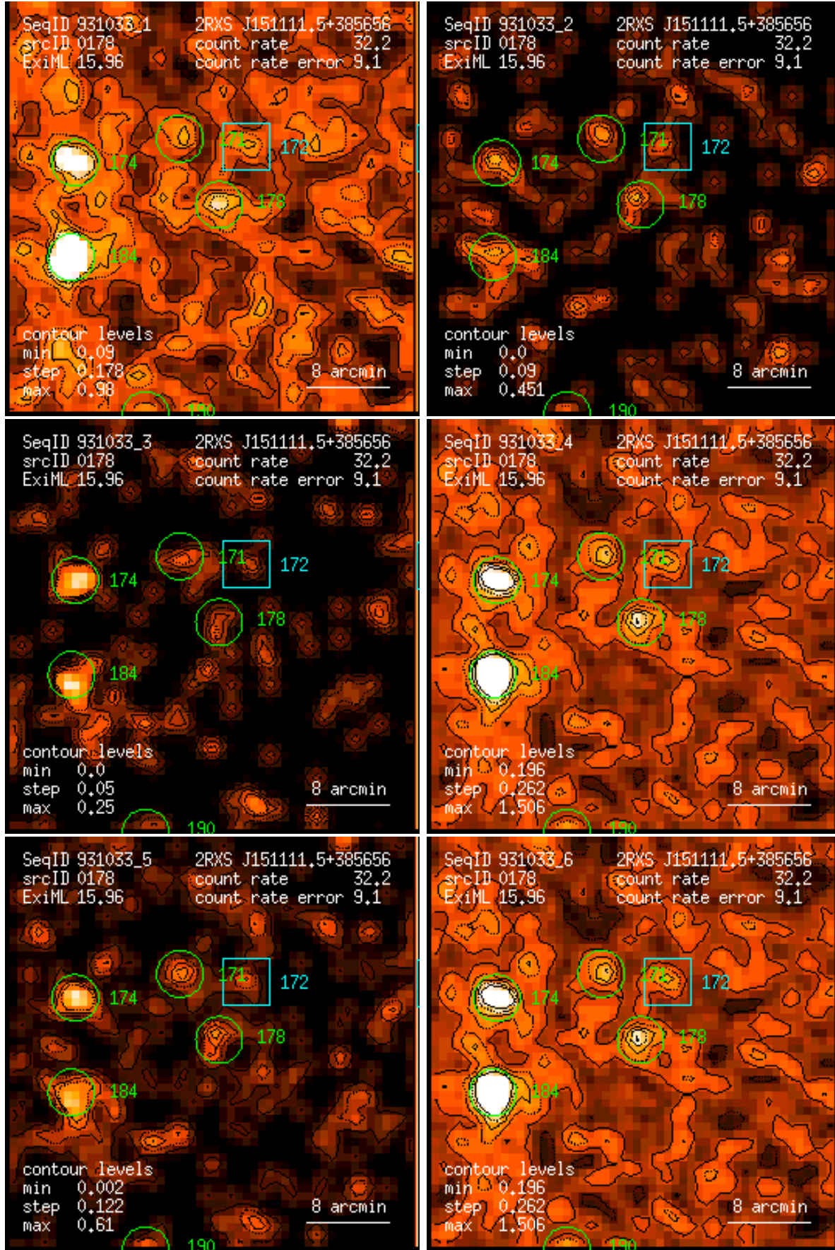
Figure 178: RASS 931033: detection 0178: band rate images, Gaussian filter: (1) PSPC channels 11 – 41, (2) 52 – 90, (3) 91 – 201, (4) 11 – 235, (5) 52 – 201, (6) 11 – 201. Broad band rates in counts/ks. Band rate contour levels in counts/ks/arcmin 2 .
