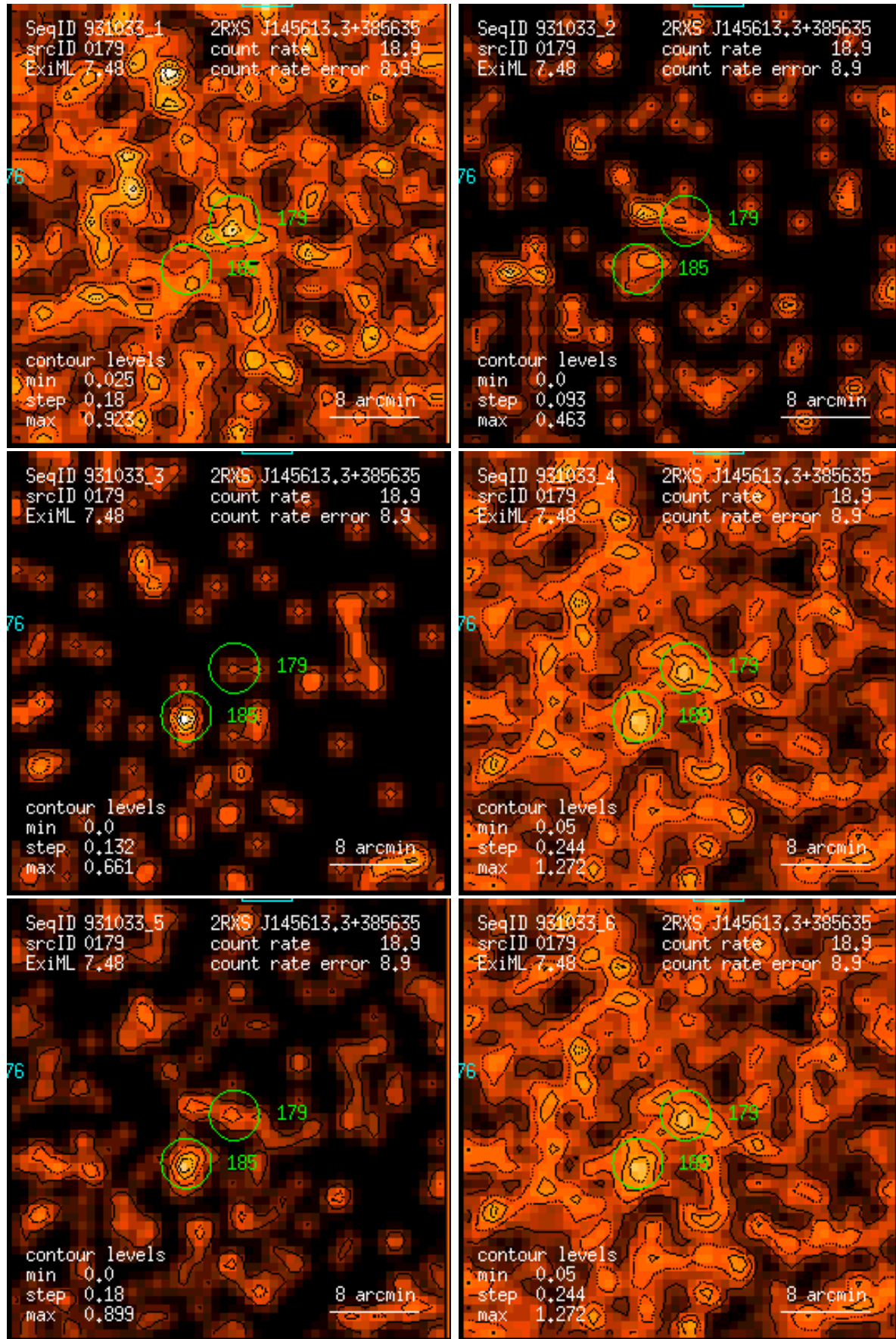
Figure 179: RASS 931033: detection 0179: band rate images, Gaussian filter: (1) PSPC channels 11 – 41, (2) 52 – 90, (3) 91 – 201, (4) 11 – 235, (5) 52 – 201, (6) 11 – 201. Broad band rates in counts/ks. Band rate contour levels in counts/ks/arcmin 2 .
