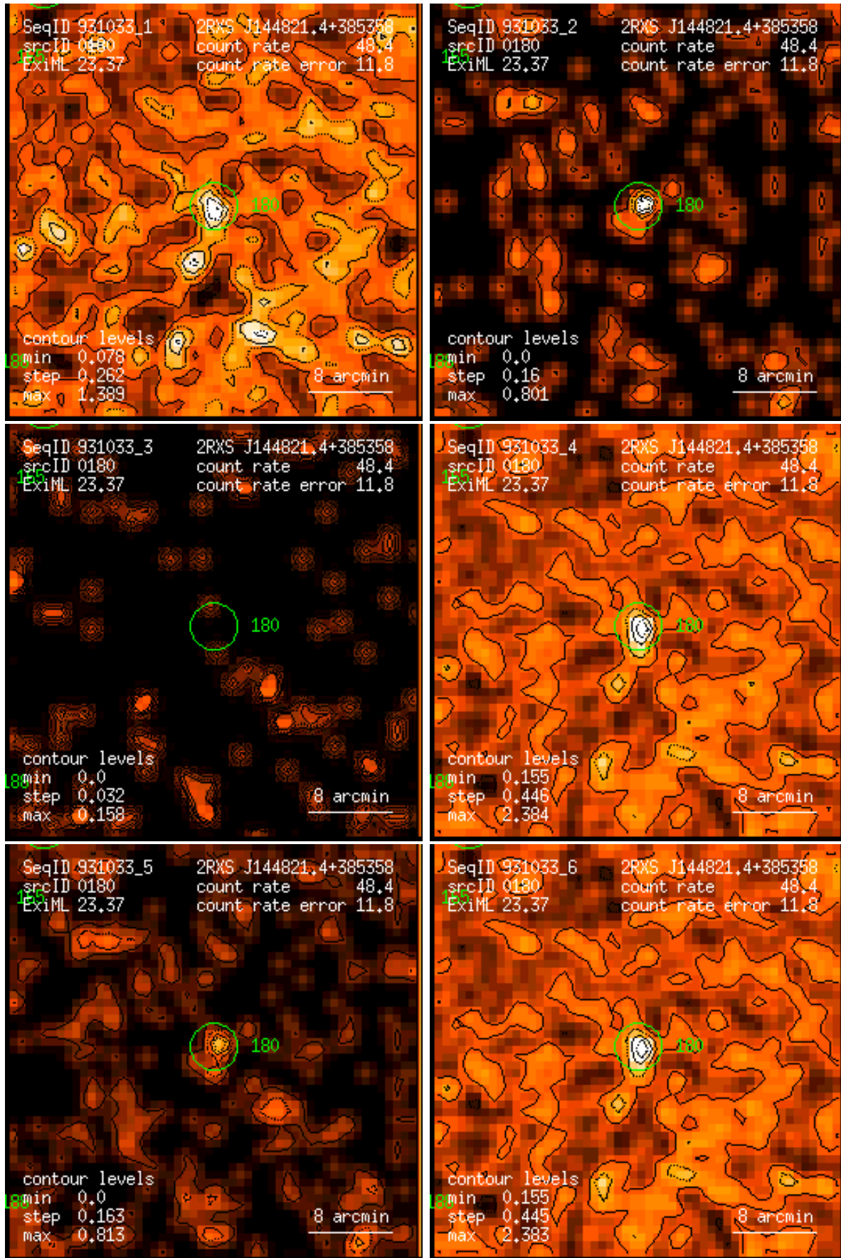
Figure 180: RASS 931033: detection 0180: band rate images, Gaussian filter: (1) PSPC channels 11 – 41, (2) 52 – 90, (3) 91 – 201, (4) 11 – 235, (5) 52 – 201, (6) 11 – 201. Broad band rates in counts/ks. Band rate contour levels in counts/ks/arcmin 2 .
