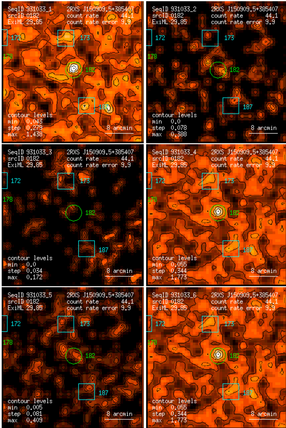
Figure 182: RASS 931033: detection 0182: band rate images, Gaussian filter: (1) PSPC channels 11 – 41, (2) 52 – 90, (3) 91 – 201, (4) 11 – 235, (5) 52 – 201, (6) 11 – 201. Broad band rates in counts/ks. Band rate contour levels in counts/ks/arcmin 2 .
