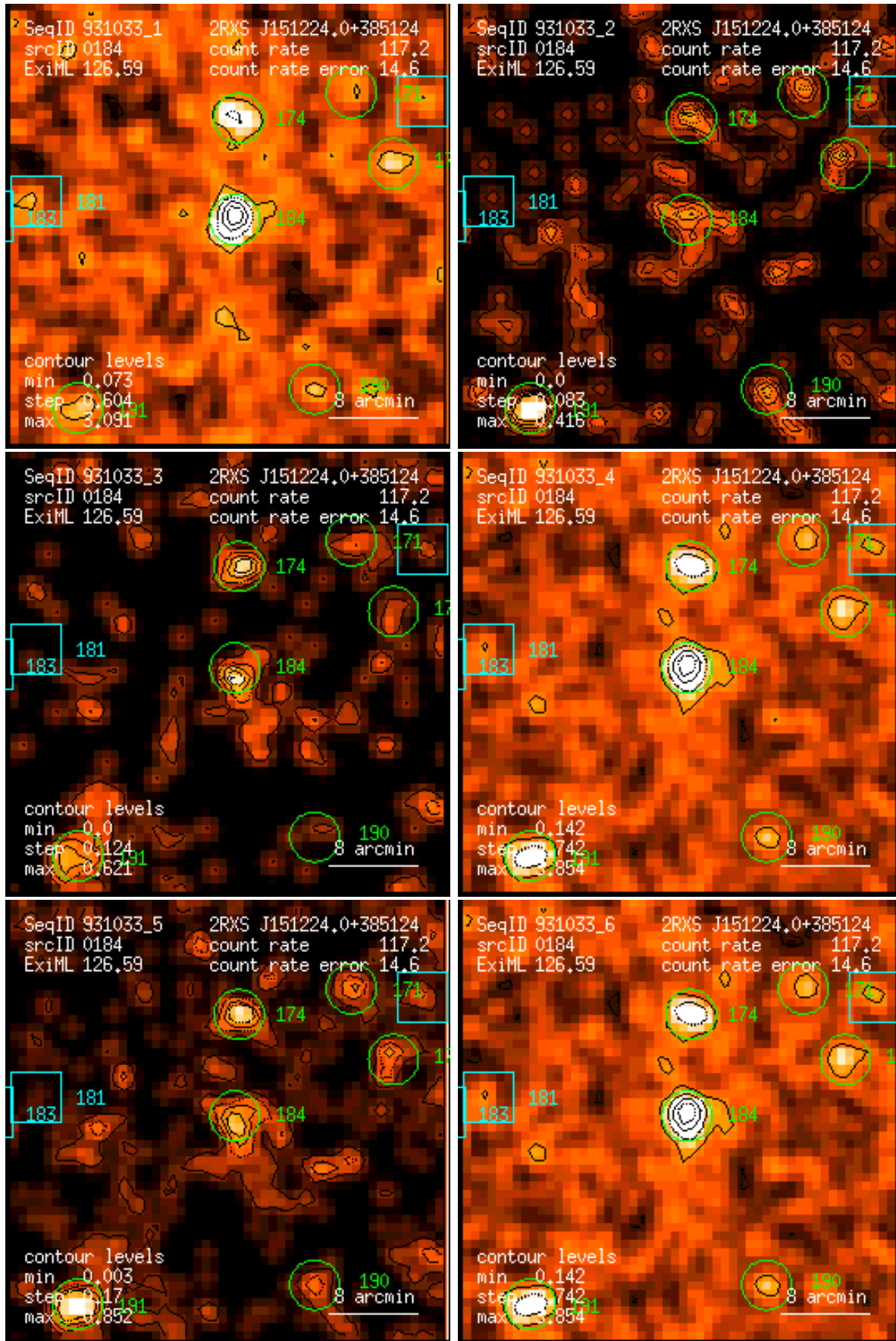
Figure 184: RASS 931033: detection 0184: band rate images, Gaussian filter: (1) PSPC channels 11 – 41, (2) 52 – 90, (3) 91 – 201, (4) 11 – 235, (5) 52 – 201, (6) 11 – 201. Broad band rates in counts/ks. Band rate contour levels in counts/ks/arcmin 2 .
