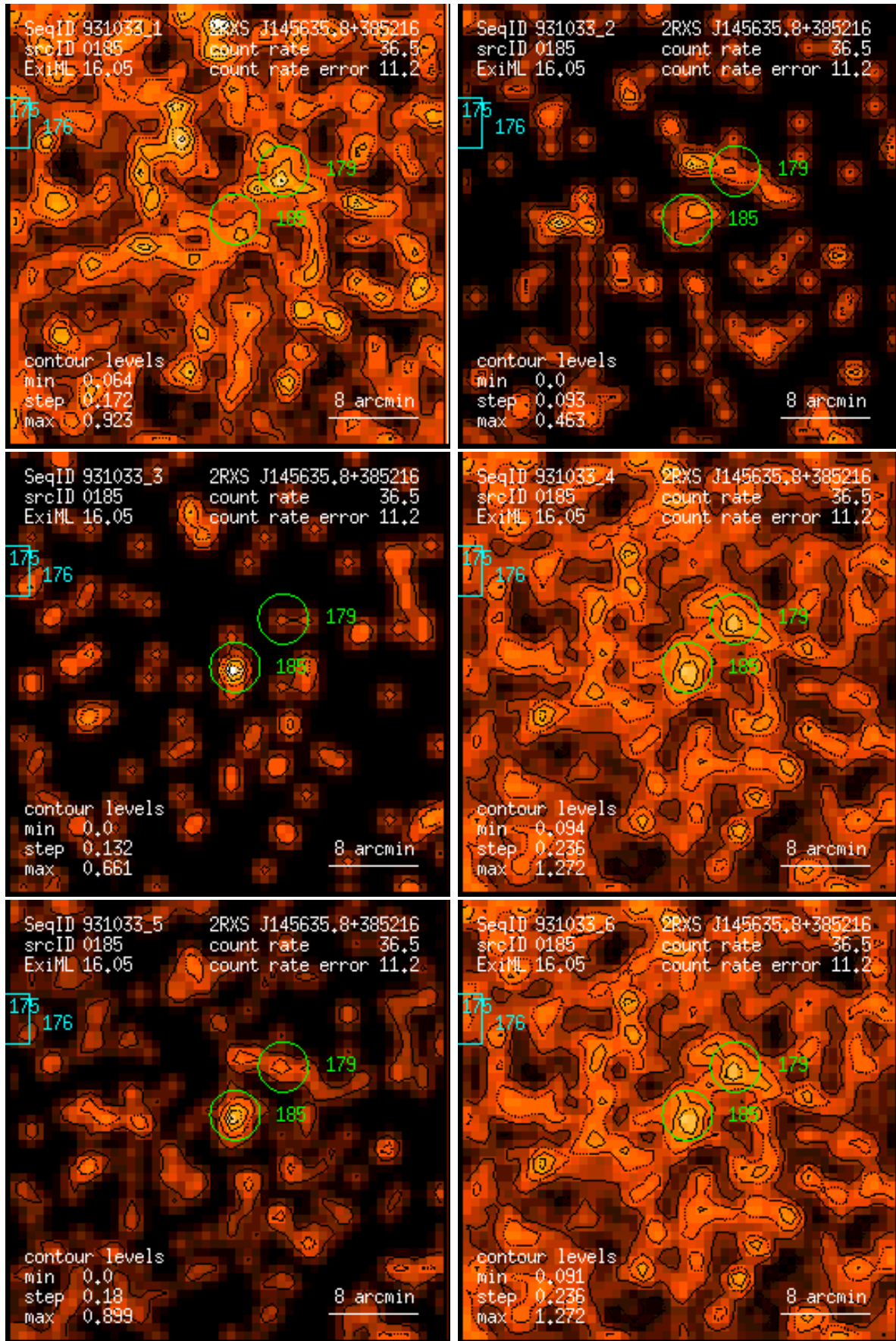
Figure 185: RASS 931033: detection 0185: band rate images, Gaussian filter: (1) PSPC channels 11 – 41, (2) 52 – 90, (3) 91 – 201, (4) 11 – 235, (5) 52 – 201, (6) 11 – 201. Broad band rates in counts/ks. Band rate contour levels in counts/ks/arcmin 2 .
