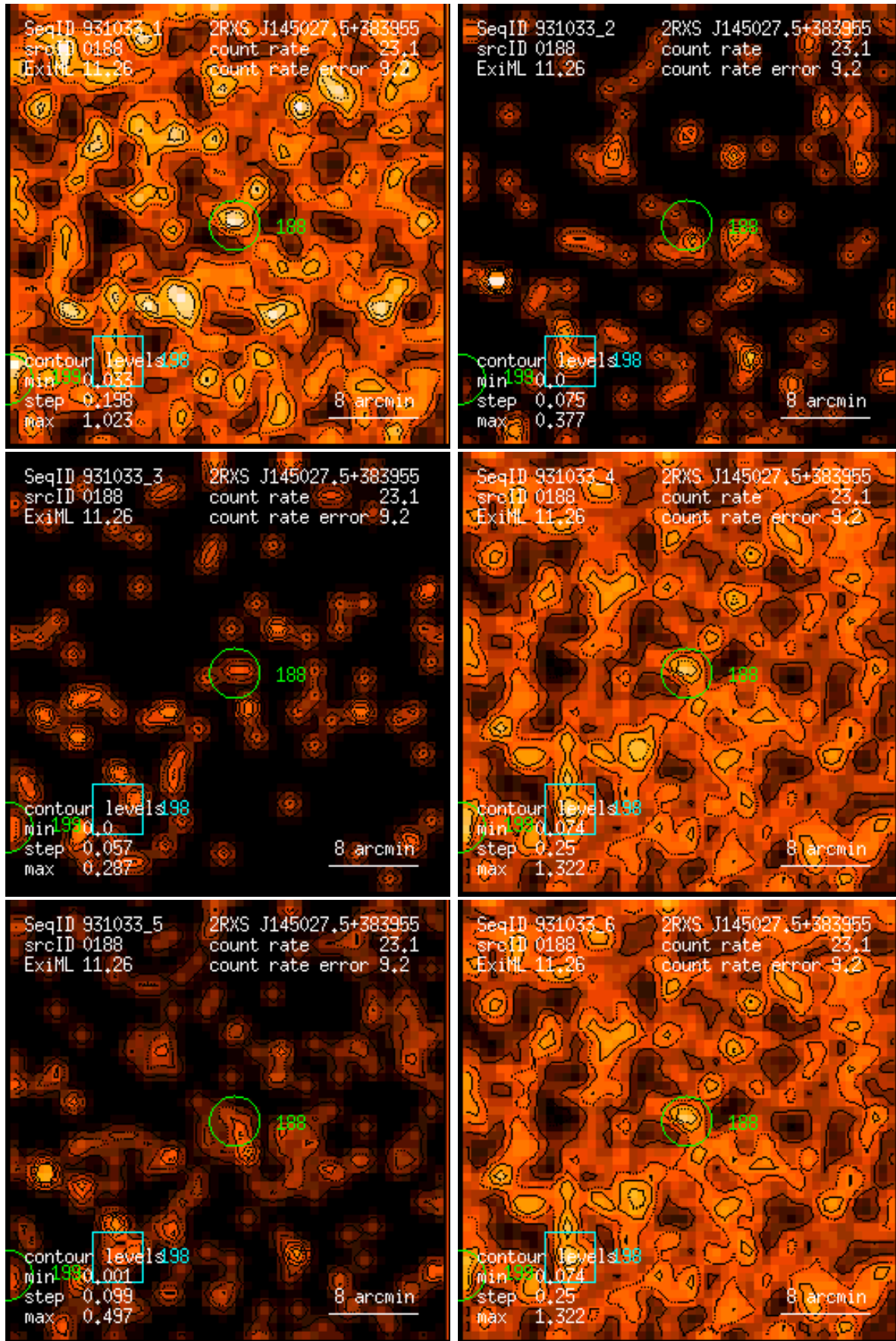
Figure 188: RASS 931033: detection 0188: band rate images, Gaussian filter: (1) PSPC channels 11 – 41, (2) 52 – 90, (3) 91 – 201, (4) 11 – 235, (5) 52 – 201, (6) 11 – 201. Broad band rates in counts/ks. Band rate contour levels in counts/ks/arcmin 2 .
