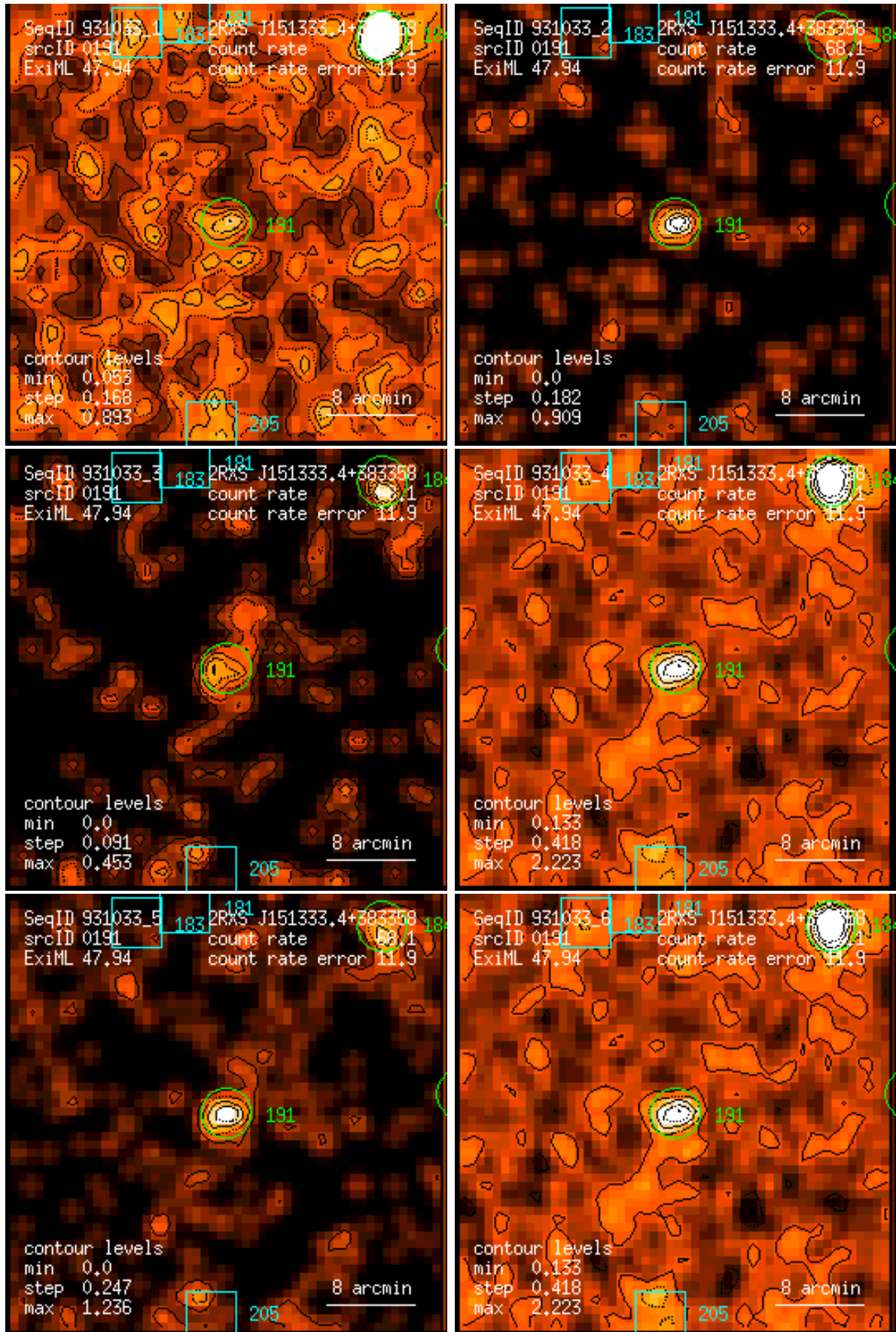
Figure 191: RASS 931033: detection 0191: band rate images, Gaussian filter: (1) PSPC channels 11 – 41, (2) 52 – 90, (3) 91 – 201, (4) 11 – 235, (5) 52 – 201, (6) 11 – 201. Broad band rates in counts/ks. Band rate contour levels in counts/ks/arcmin 2 .
