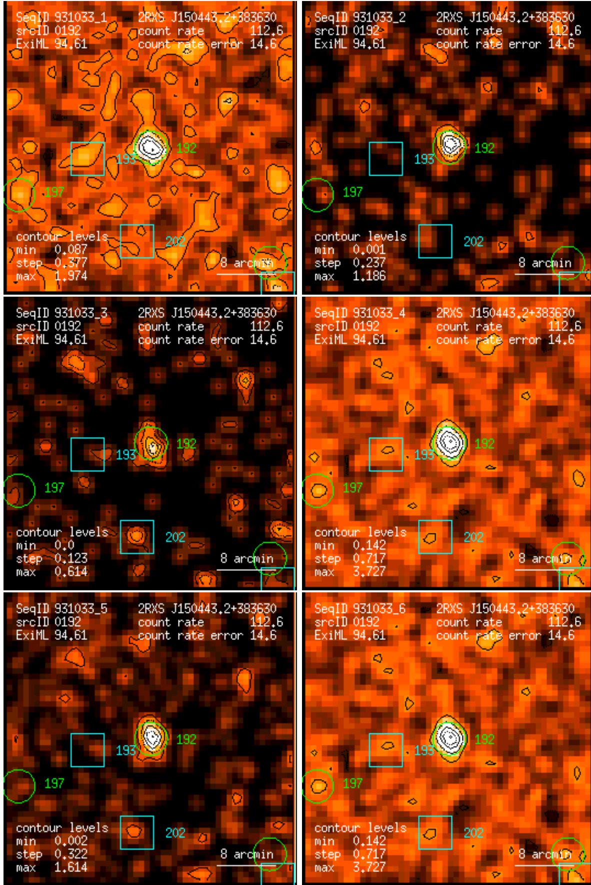
Figure 192: RASS 931033: detection 0192: band rate images, Gaussian filter: (1) PSPC channels 11 – 41, (2) 52 – 90, (3) 91 – 201, (4) 11 – 235, (5) 52 – 201, (6) 11 – 201. Broad band rates in counts/ks. Band rate contour levels in counts/ks/arcmin 2 .
