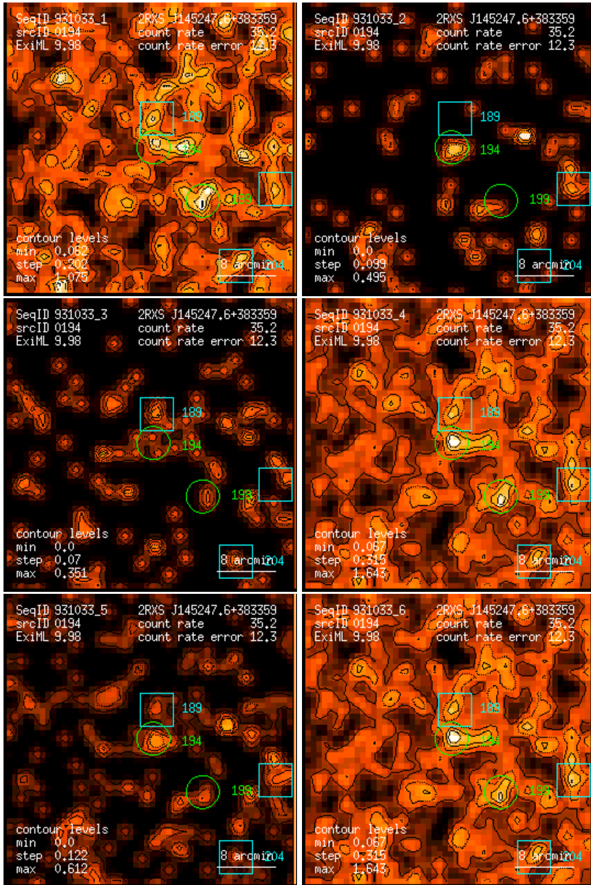
Figure 194: RASS 931033: detection 0194: band rate images, Gaussian filter: (1) PSPC channels 11 – 41, (2) 52 – 90, (3) 91 – 201, (4) 11 – 235, (5) 52 – 201, (6) 11 – 201. Broad band rates in counts/ks. Band rate contour levels in counts/ks/arcmin 2 .
