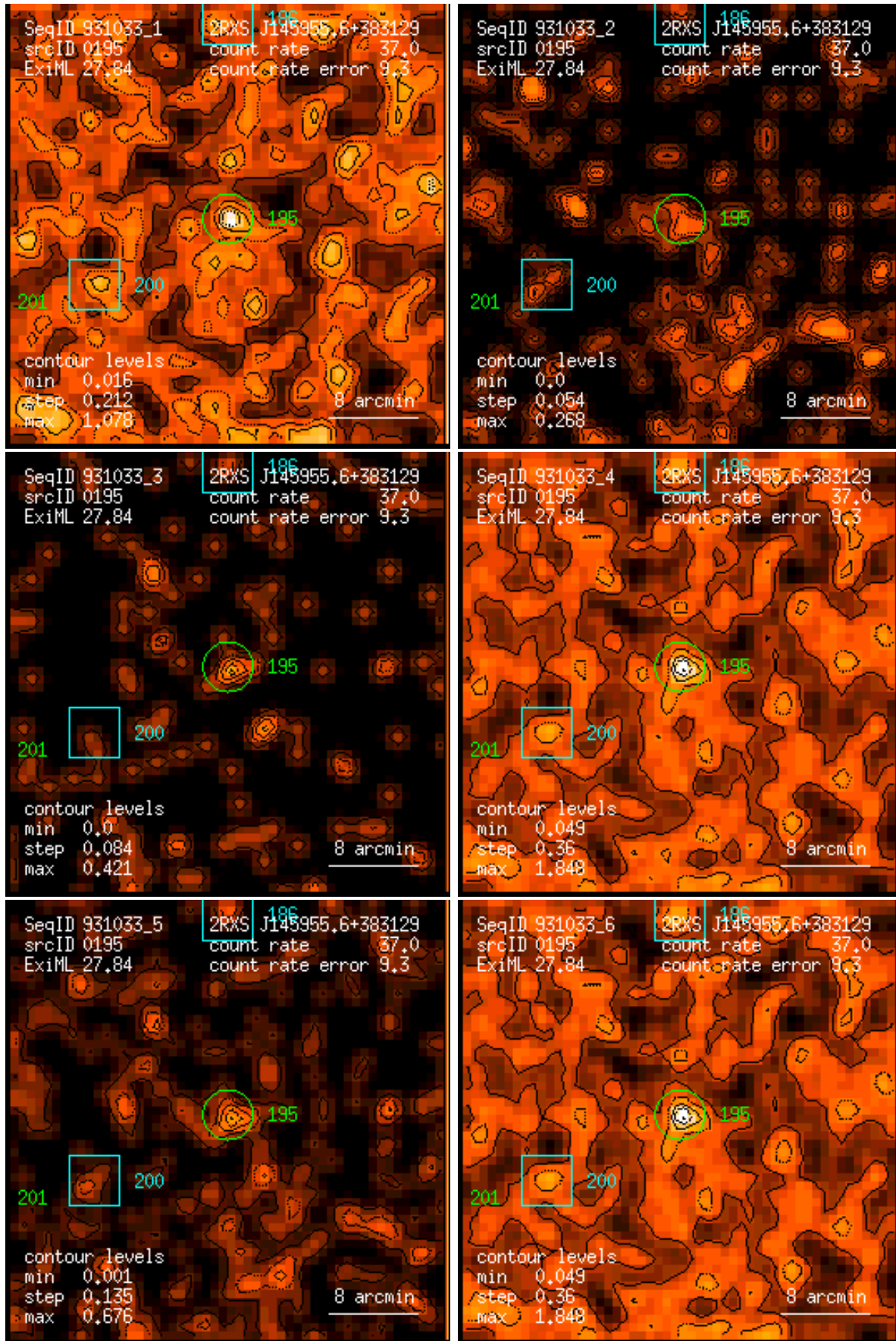
Figure 195: RASS 931033: detection 0195: band rate images, Gaussian filter: (1) PSPC channels 11 – 41, (2) 52 – 90, (3) 91 – 201, (4) 11 – 235, (5) 52 – 201, (6) 11 – 201. Broad band rates in counts/ks. Band rate contour levels in counts/ks/arcmin 2 .
