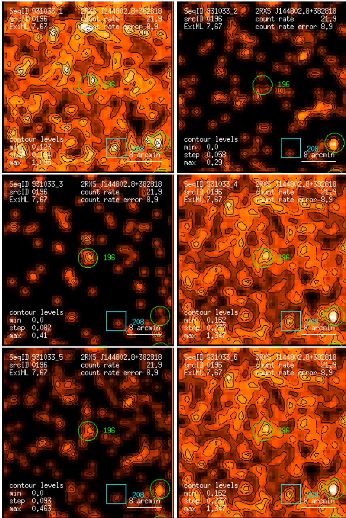
Figure 196: RASS 931033: detection 0196: band rate images, Gaussian filter: (1) PSPC channels 11 – 41, (2) 52 – 90, (3) 91 – 201, (4) 11 – 235, (5) 52 – 201, (6) 11 – 201. Broad band rates in counts/ks. Band rate contour levels in counts/ks/arcmin 2 .
