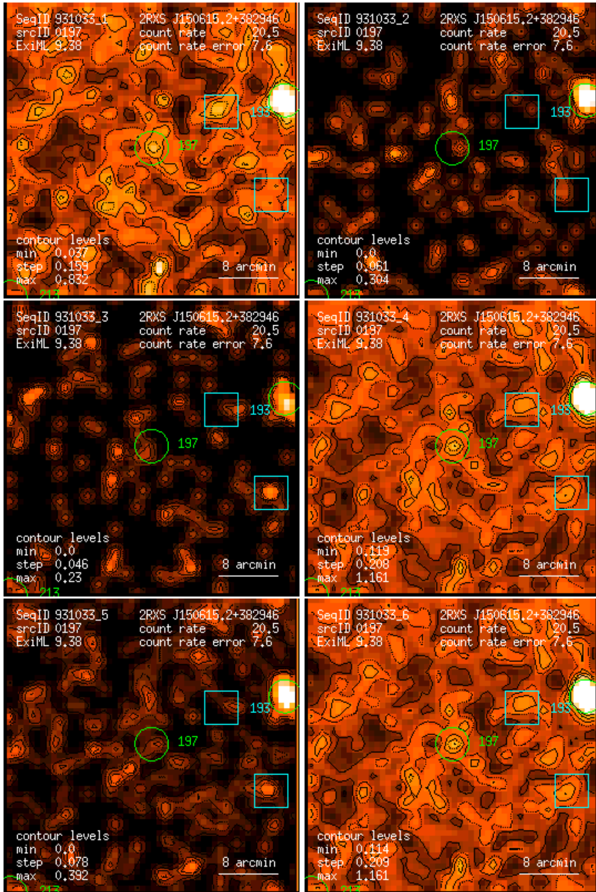
Figure 197: RASS 931033: detection 0197: band rate images, Gaussian filter: (1) PSPC channels 11 – 41, (2) 52 – 90, (3) 91 – 201, (4) 11 – 235, (5) 52 – 201, (6) 11 – 201. Broad band rates in counts/ks. Band rate contour levels in counts/ks/arcmin 2 .
