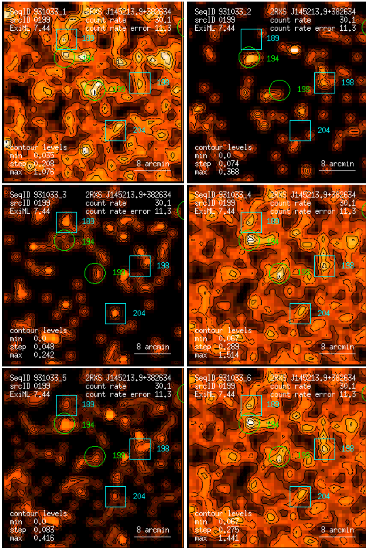
Figure 199: RASS 931033: detection 0199: band rate images, Gaussian filter: (1) PSPC channels 11 – 41, (2) 52 – 90, (3) 91 – 201, (4) 11 – 235, (5) 52 – 201, (6) 11 – 201. Broad band rates in counts/ks. Band rate contour levels in counts/ks/arcmin 2 .
