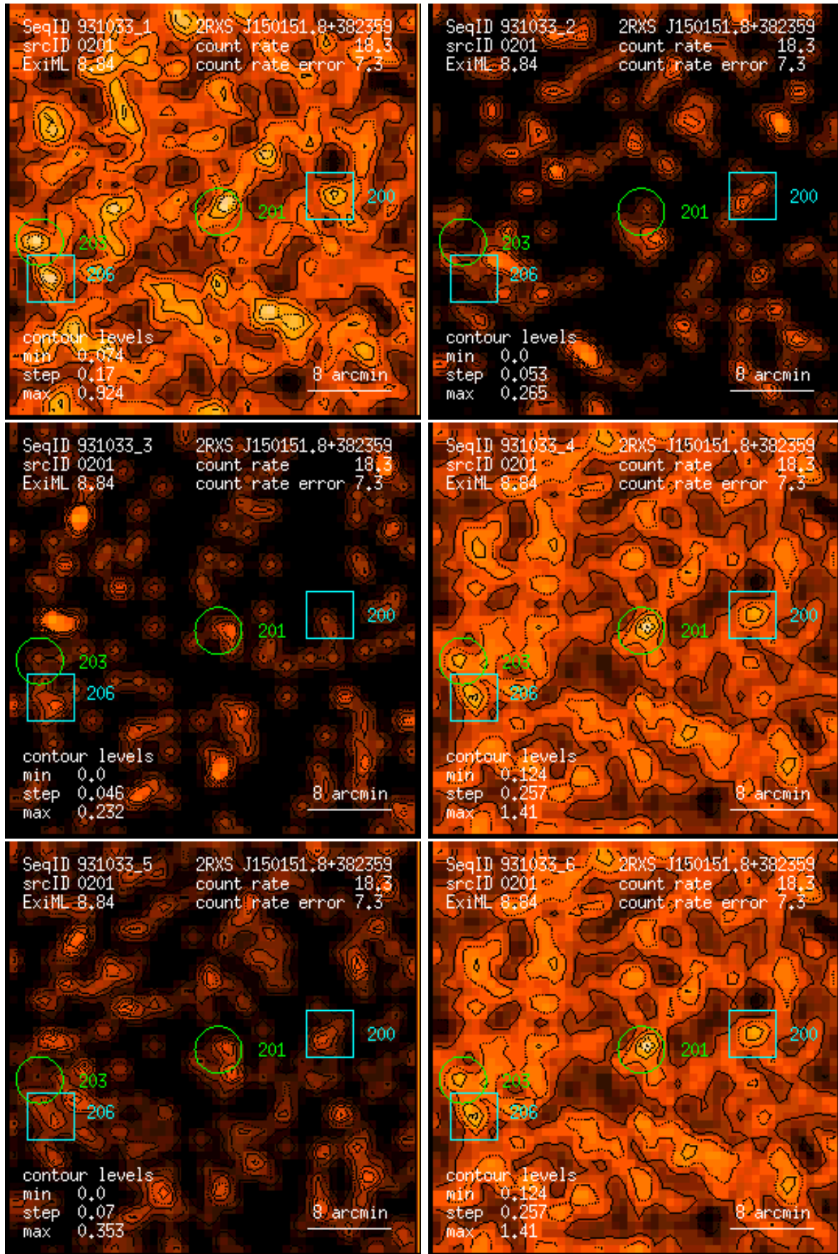
Figure 201: RASS 931033: detection 0201: band rate images, Gaussian filter: (1) PSPC channels 11 – 41, (2) 52 – 90, (3) 91 – 201, (4) 11 – 235, (5) 52 – 201, (6) 11 – 201. Broad band rates in counts/ks. Band rate contour levels in counts/ks/arcmin 2 .
