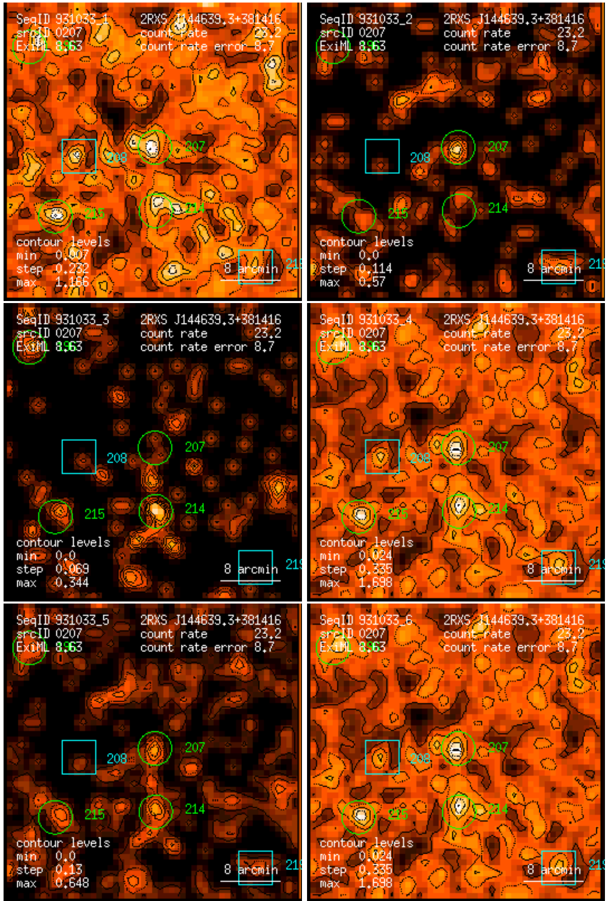
Figure 207: RASS 931033: detection 0207: band rate images, Gaussian filter: (1) PSPC channels 11 – 41, (2) 52 – 90, (3) 91 – 201, (4) 11 – 235, (5) 52 – 201, (6) 11 – 201. Broad band rates in counts/ks. Band rate contour levels in counts/ks/arcmin 2 .
