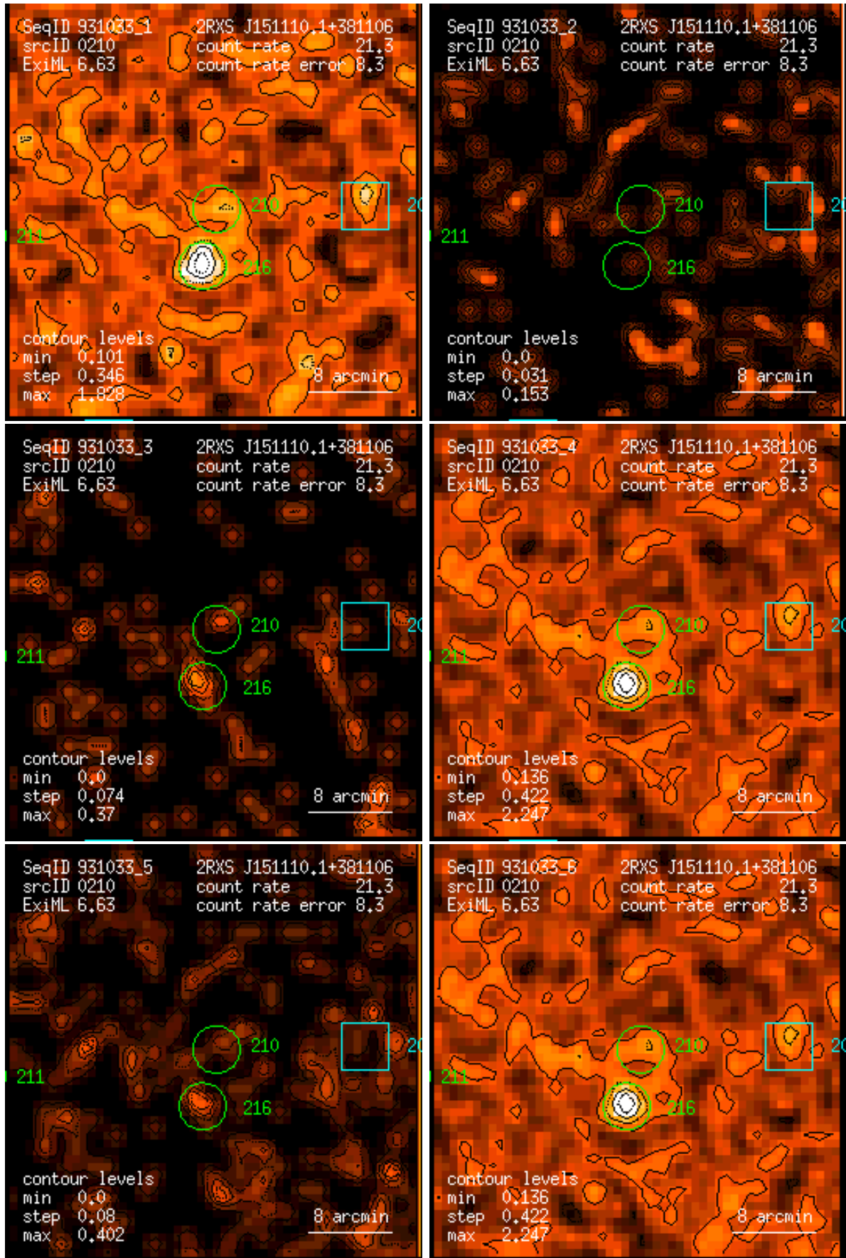
Figure 210: RASS 931033: detection 0210: band rate images, Gaussian filter: (1) PSPC channels 11 – 41, (2) 52 – 90, (3) 91 – 201, (4) 11 – 235, (5) 52 – 201, (6) 11 – 201. Broad band rates in counts/ks. Band rate contour levels in counts/ks/arcmin 2 .
