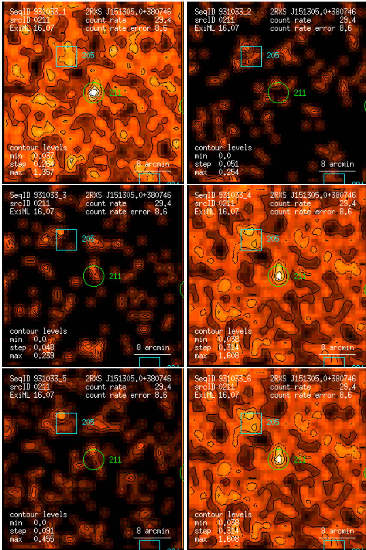
Figure 211: RASS 931033: detection 0211: band rate images, Gaussian filter: (1) PSPC channels 11 – 41, (2) 52 – 90, (3) 91 – 201, (4) 11 – 235, (5) 52 – 201, (6) 11 – 201. Broad band rates in counts/ks. Band rate contour levels in counts/ks/arcmin 2 .
