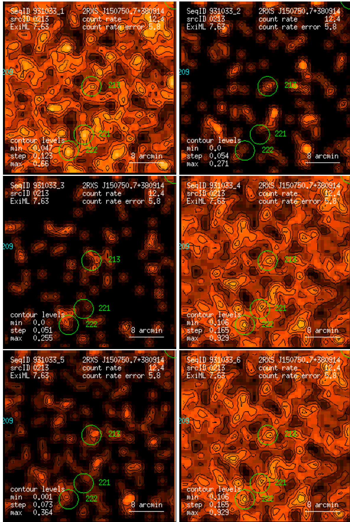
Figure 213: RASS 931033: detection 0213: band rate images, Gaussian filter: (1) PSPC channels 11 – 41, (2) 52 – 90, (3) 91 – 201, (4) 11 – 235, (5) 52 – 201, (6) 11 – 201. Broad band rates in counts/ks. Band rate contour levels in counts/ks/arcmin 2 .
