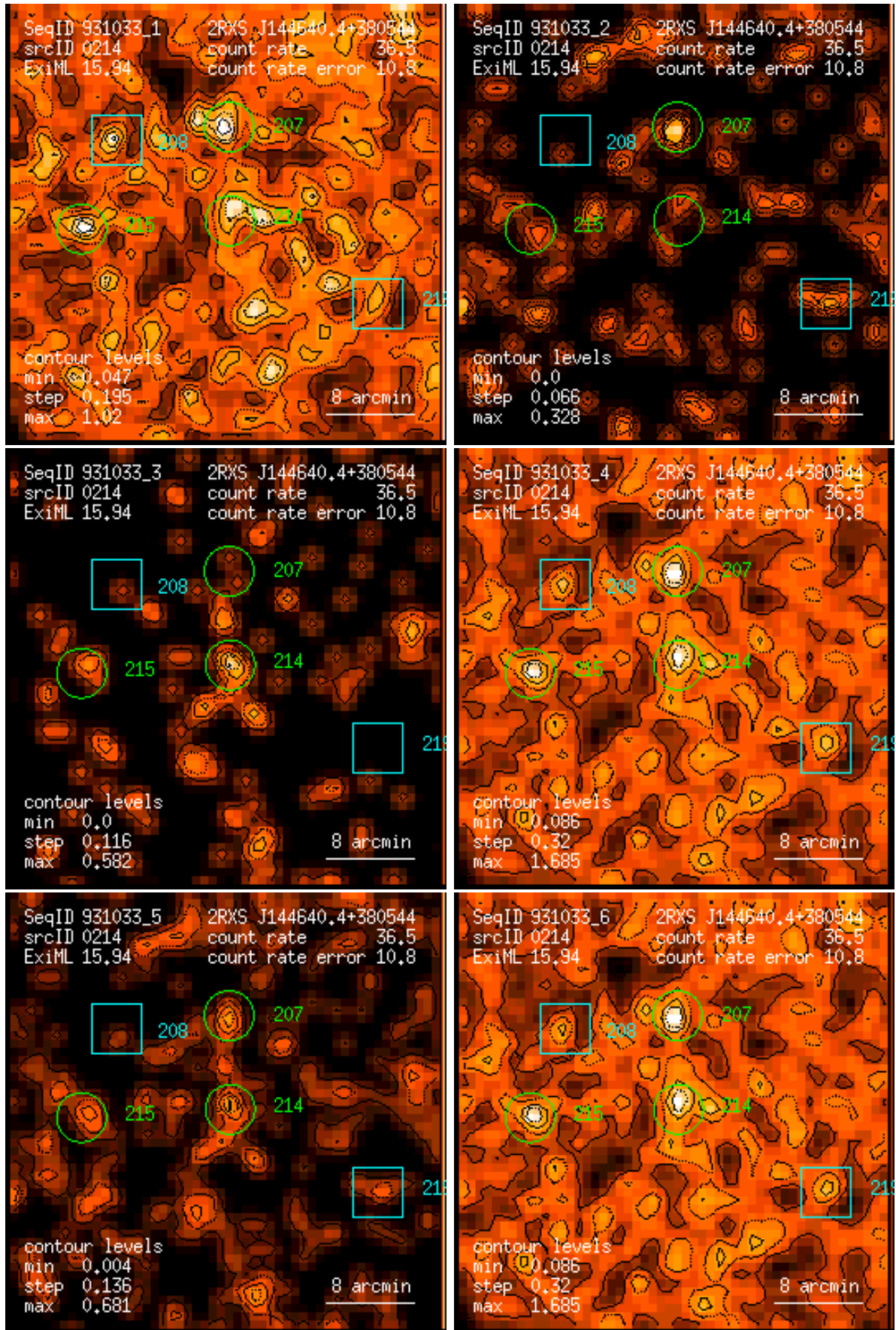
Figure 214: RASS 931033: detection 0214: band rate images, Gaussian filter: (1) PSPC channels 11 – 41, (2) 52 – 90, (3) 91 – 201, (4) 11 – 235, (5) 52 – 201, (6) 11 – 201. Broad band rates in counts/ks. Band rate contour levels in counts/ks/arcmin 2 .
