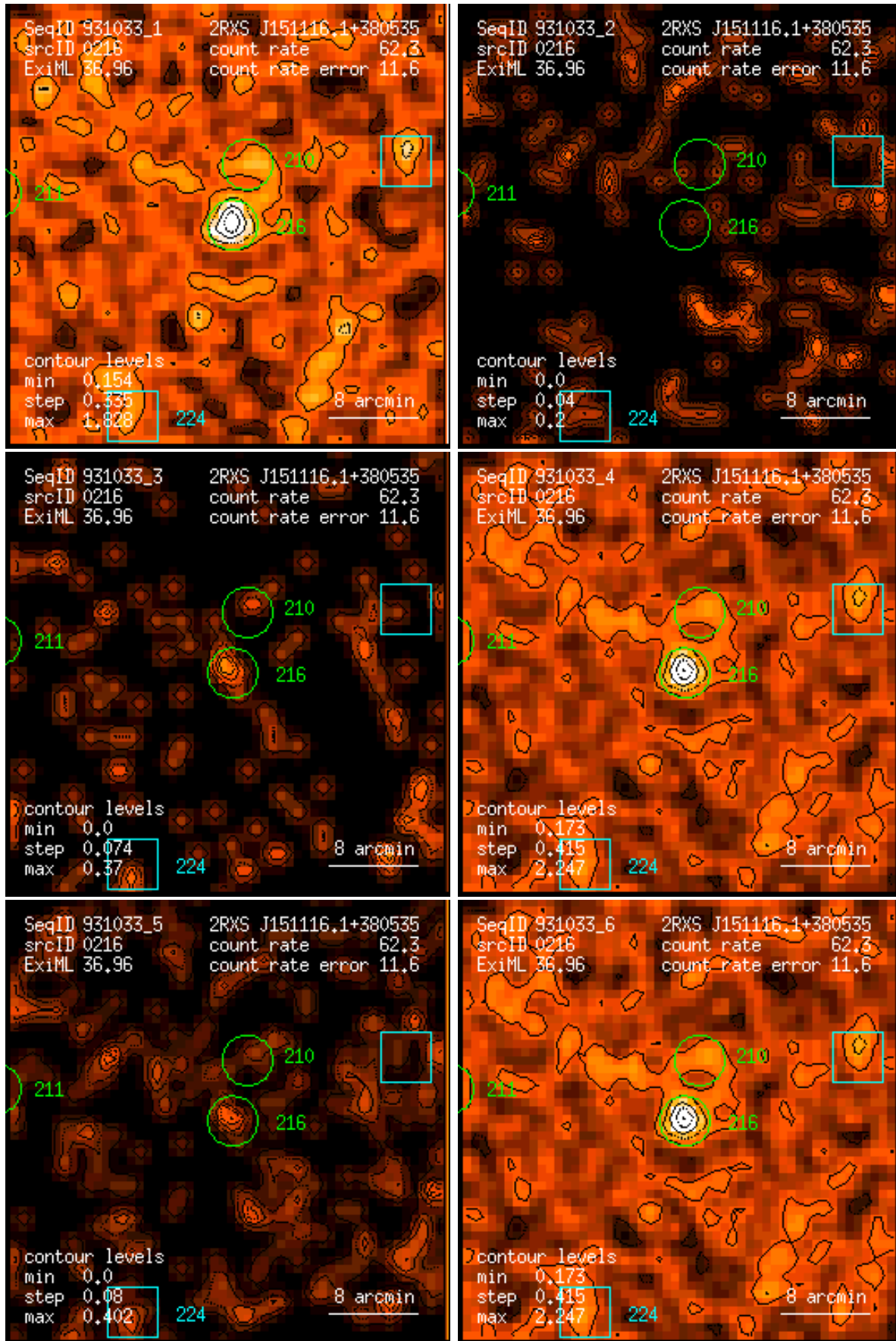
Figure 216: RASS 931033: detection 0216: band rate images, Gaussian filter: (1) PSPC channels 11 – 41, (2) 52 – 90, (3) 91 – 201, (4) 11 – 235, (5) 52 – 201, (6) 11 – 201. Broad band rates in counts/ks. Band rate contour levels in counts/ks/arcmin 2 .
