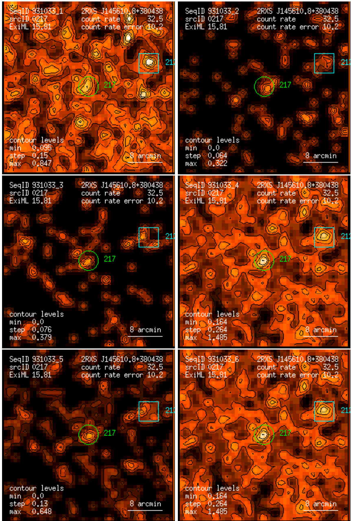
Figure 217: RASS 931033: detection 0217: band rate images, Gaussian filter: (1) PSPC channels 11 – 41, (2) 52 – 90, (3) 91 – 201, (4) 11 – 235, (5) 52 – 201, (6) 11 – 201. Broad band rates in counts/ks. Band rate contour levels in counts/ks/arcmin 2 .
