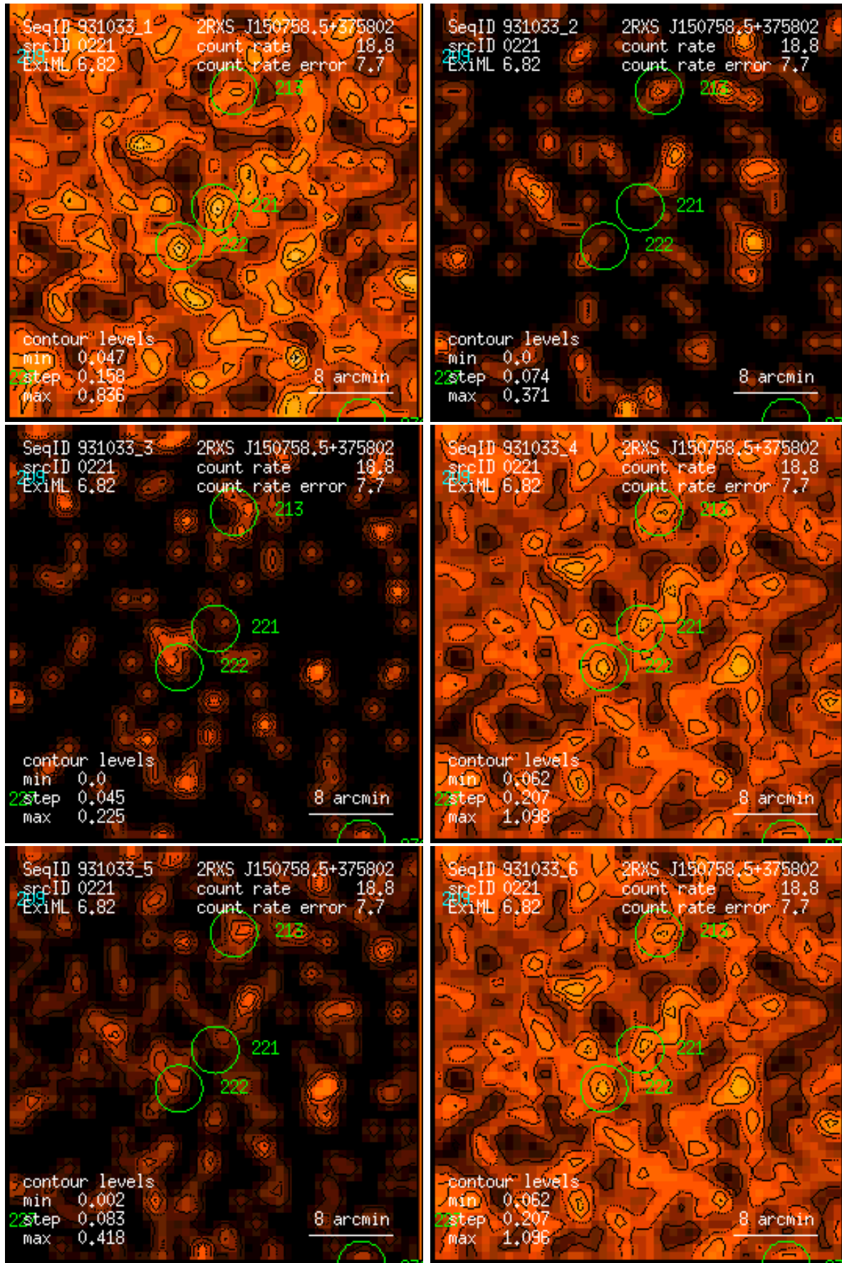
Figure 221: RASS 931033: detection 0221: band rate images, Gaussian filter: (1) PSPC channels 11 – 41, (2) 52 – 90, (3) 91 – 201, (4) 11 – 235, (5) 52 – 201, (6) 11 – 201. Broad band rates in counts/ks. Band rate contour levels in counts/ks/arcmin 2 .
