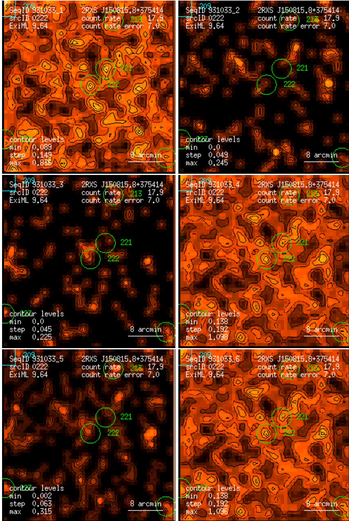
Figure 222: RASS 931033: detection 0222: band rate images, Gaussian filter: (1) PSPC channels 11 – 41, (2) 52 – 90, (3) 91 – 201, (4) 11 – 235, (5) 52 – 201, (6) 11 – 201. Broad band rates in counts/ks. Band rate contour levels in counts/ks/arcmin 2 .
