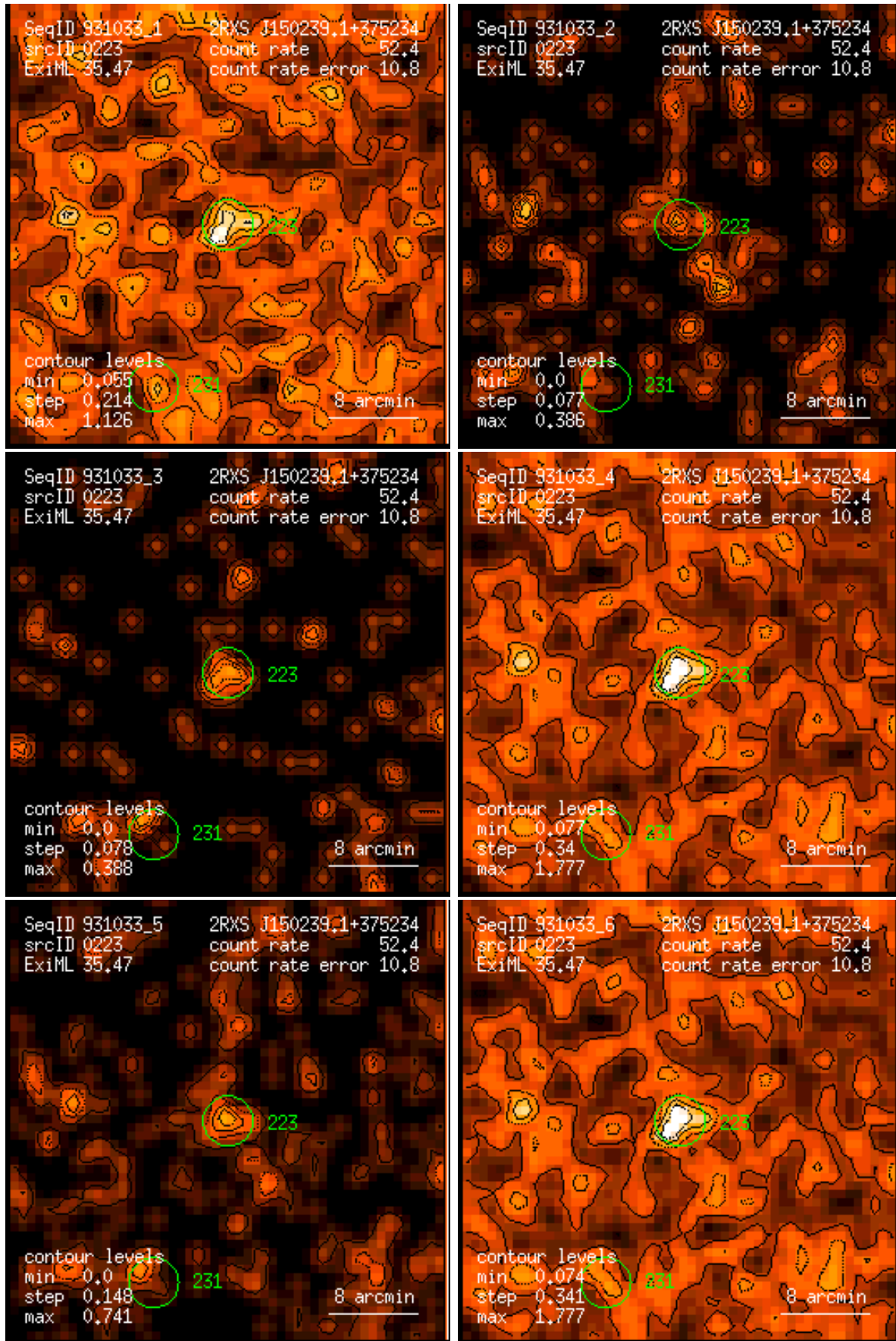
Figure 223: RASS 931033: detection 0223: band rate images, Gaussian filter: (1) PSPC channels 11 – 41, (2) 52 – 90, (3) 91 – 201, (4) 11 – 235, (5) 52 – 201, (6) 11 – 201. Broad band rates in counts/ks. Band rate contour levels in counts/ks/arcmin 2 .
