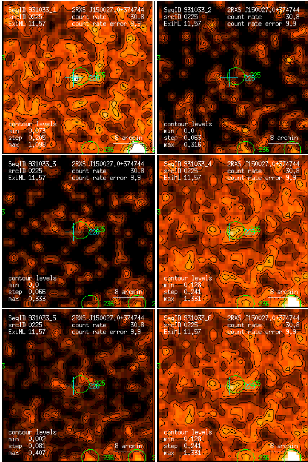
Figure 225: RASS 931033: detection 0225: band rate images, Gaussian filter: (1) PSPC channels 11 – 41, (2) 52 – 90, (3) 91 – 201, (4) 11 – 235, (5) 52 – 201, (6) 11 – 201. Broad band rates in counts/ks. Band rate contour levels in counts/ks/arcmin 2 .
