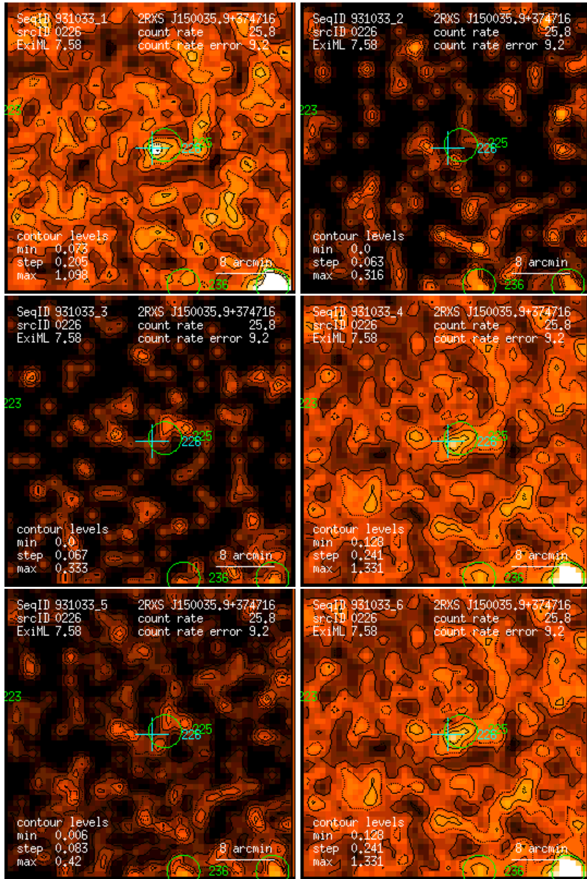
Figure 226: RASS 931033: detection 0226: band rate images, Gaussian filter: (1) PSPC channels 11 – 41, (2) 52 – 90, (3) 91 – 201, (4) 11 – 235, (5) 52 – 201, (6) 11 – 201. Broad band rates in counts/ks. Band rate contour levels in counts/ks/arcmin 2 .
