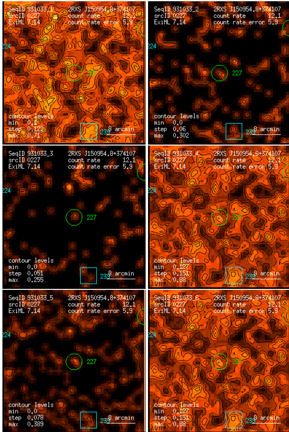
Figure 227: RASS 931033: detection 0227: band rate images, Gaussian filter: (1) PSPC channels 11 – 41, (2) 52 – 90, (3) 91 – 201, (4) 11 – 235, (5) 52 – 201, (6) 11 – 201. Broad band rates in counts/ks. Band rate contour levels in counts/ks/arcmin 2 .
