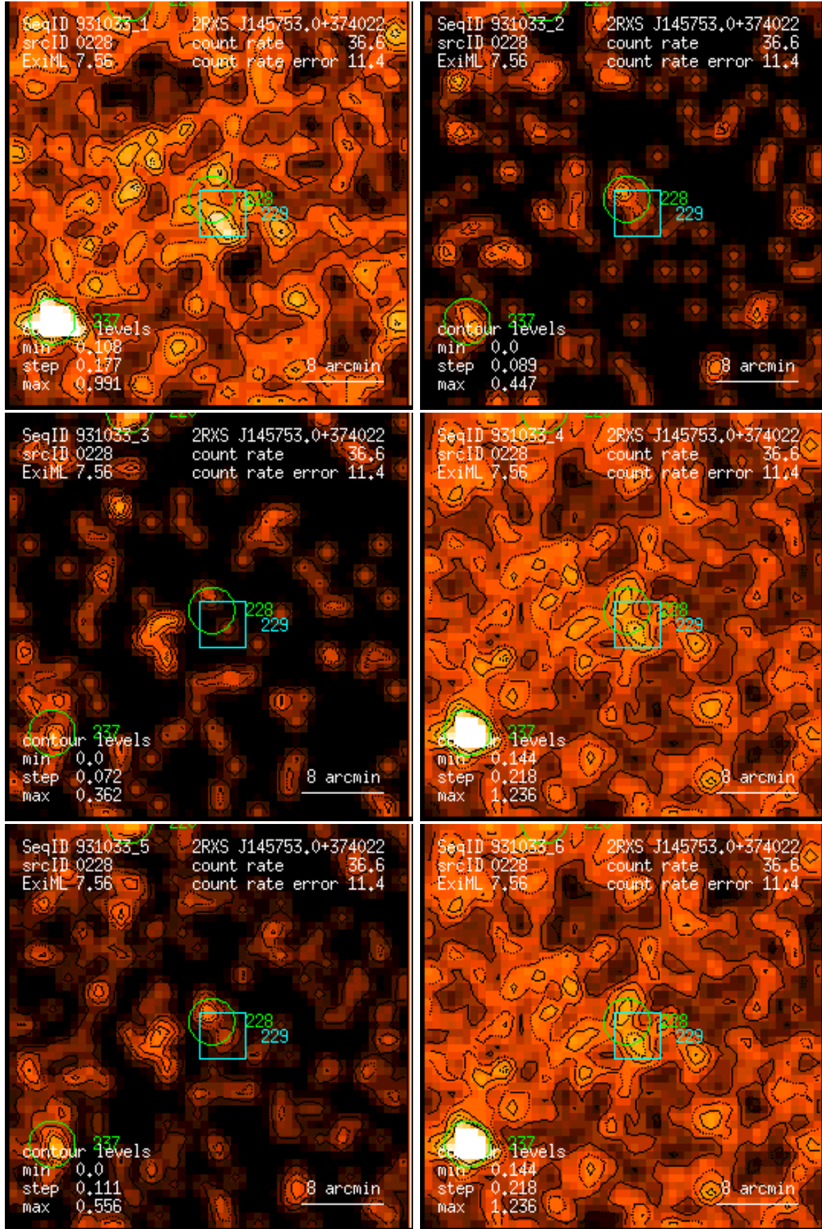
Figure 228: RASS 931033: detection 0228: band rate images, Gaussian filter: (1) PSPC channels 11 – 41, (2) 52 – 90, (3) 91 – 201, (4) 11 – 235, (5) 52 – 201, (6) 11 – 201. Broad band rates in counts/ks. Band rate contour levels in counts/ks/arcmin 2 .
