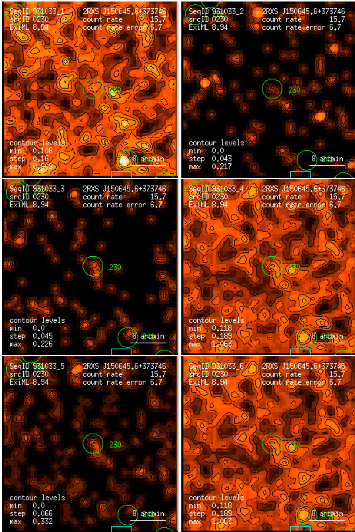
Figure 230: RASS 931033: detection 0230: band rate images, Gaussian filter: (1) PSPC channels 11 – 41, (2) 52 – 90, (3) 91 – 201, (4) 11 – 235, (5) 52 – 201, (6) 11 – 201. Broad band rates in counts/ks. Band rate contour levels in counts/ks/arcmin 2 .
