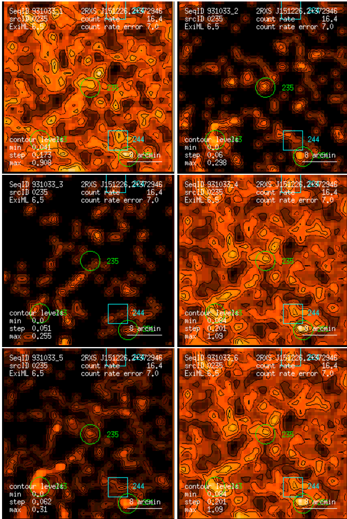
Figure 235: RASS 931033: detection 0235: band rate images, Gaussian filter: (1) PSPC channels 11 – 41, (2) 52 – 90, (3) 91 – 201, (4) 11 – 235, (5) 52 – 201, (6) 11 – 201. Broad band rates in counts/ks. Band rate contour levels in counts/ks/arcmin 2 .
