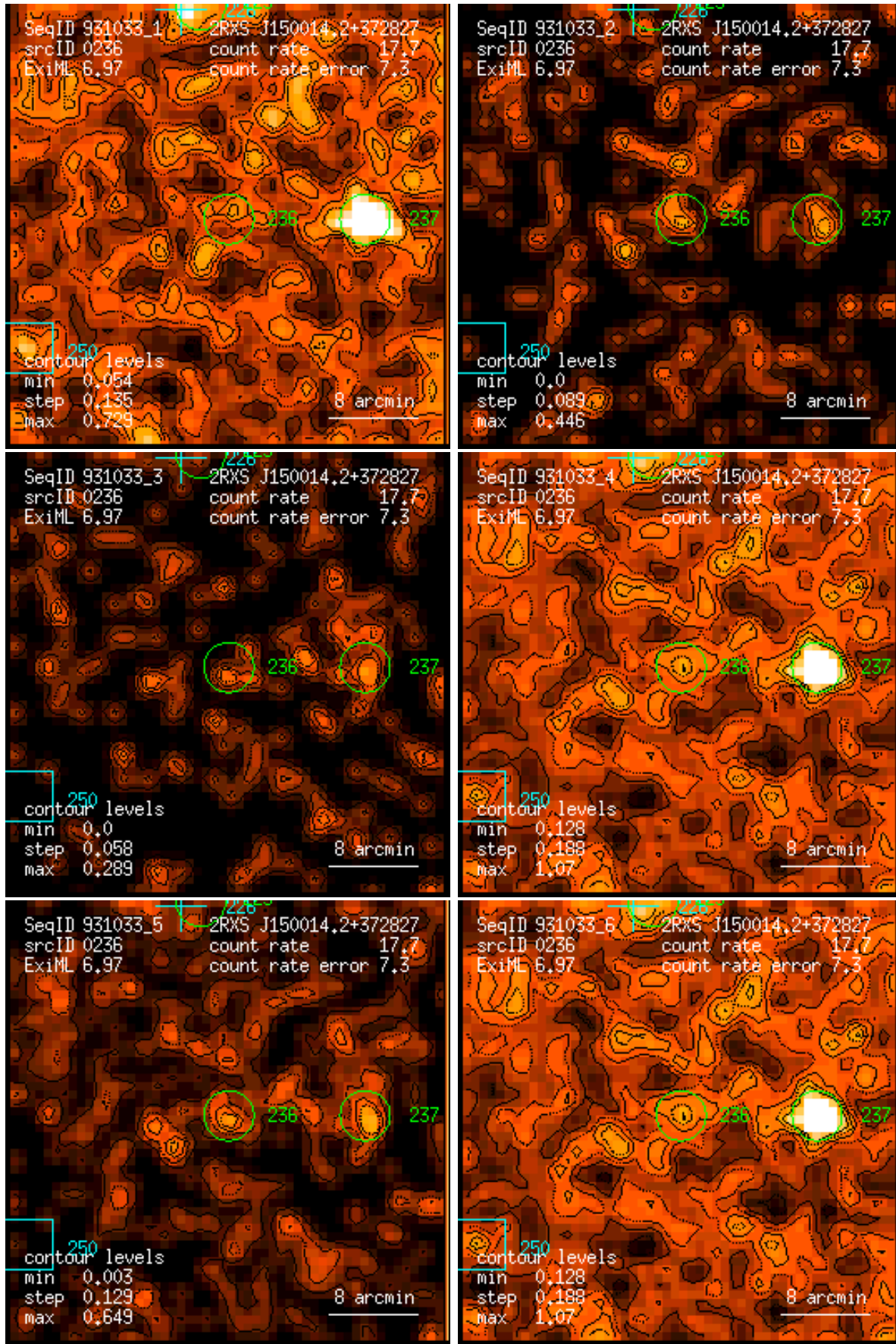
Figure 236: RASS 931033: detection 0236: band rate images, Gaussian filter: (1) PSPC channels 11 – 41, (2) 52 – 90, (3) 91 – 201, (4) 11 – 235, (5) 52 – 201, (6) 11 – 201. Broad band rates in counts/ks. Band rate contour levels in counts/ks/arcmin 2 .
