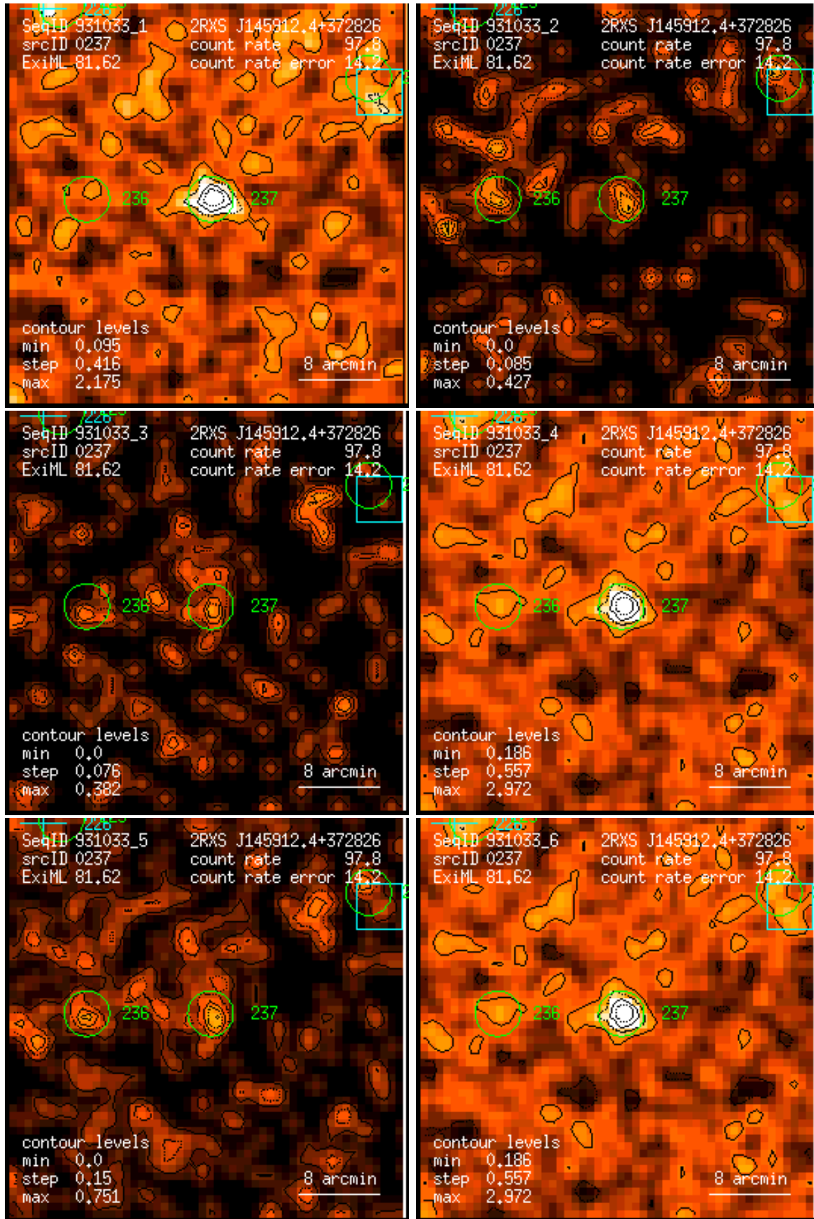
Figure 237: RASS 931033: detection 0237: band rate images, Gaussian filter: (1) PSPC channels 11 – 41, (2) 52 – 90, (3) 91 – 201, (4) 11 – 235, (5) 52 – 201, (6) 11 – 201. Broad band rates in counts/ks. Band rate contour levels in counts/ks/arcmin 2 .
