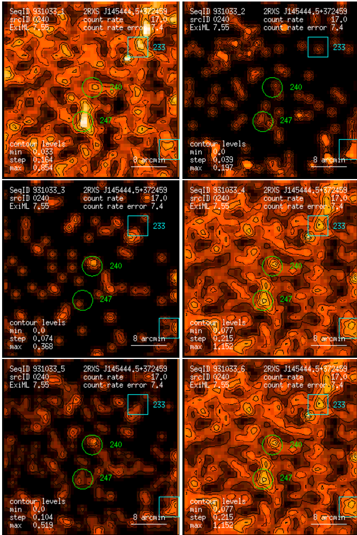
Figure 240: RASS 931033: detection 0240: band rate images, Gaussian filter: (1) PSPC channels 11 – 41, (2) 52 – 90, (3) 91 – 201, (4) 11 – 235, (5) 52 – 201, (6) 11 – 201. Broad band rates in counts/ks. Band rate contour levels in counts/ks/arcmin 2 .
