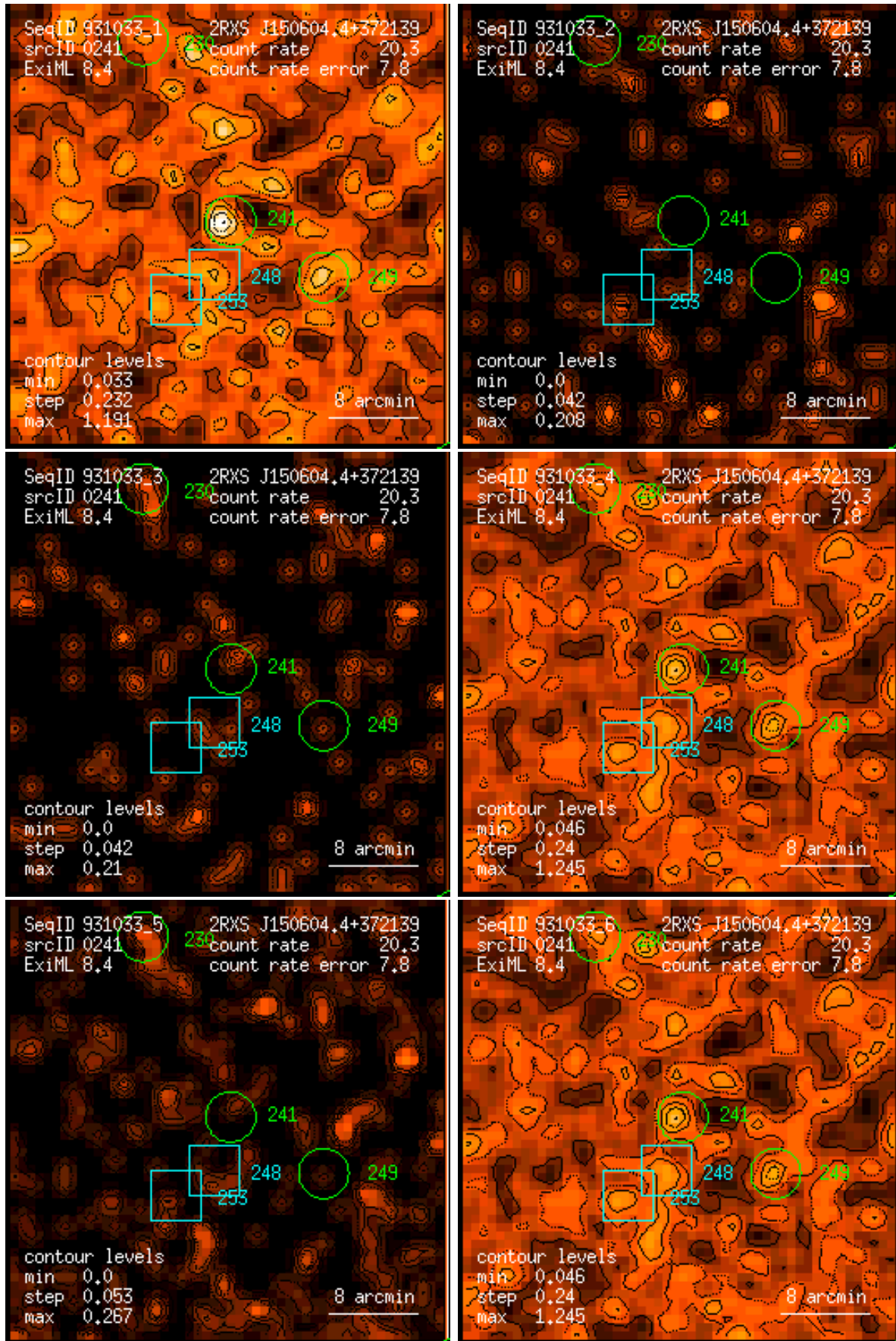
Figure 241: RASS 931033: detection 0241: band rate images, Gaussian filter: (1) PSPC channels 11 – 41, (2) 52 – 90, (3) 91 – 201, (4) 11 – 235, (5) 52 – 201, (6) 11 – 201. Broad band rates in counts/ks. Band rate contour levels in counts/ks/arcmin 2 .
